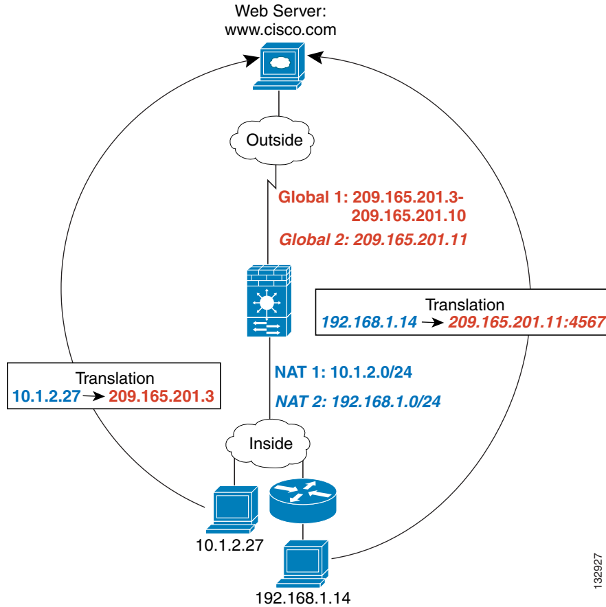
Figure 22-16 Different NAT IDs
