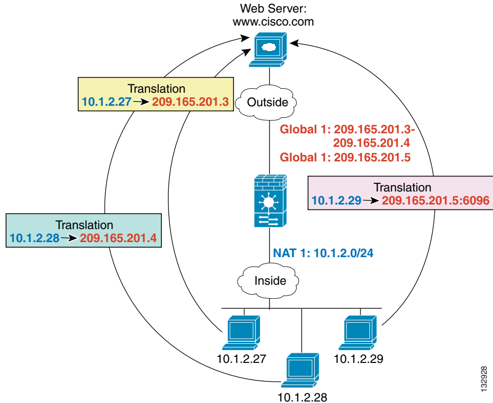
Figure 22-17 NAT and PAT Together
