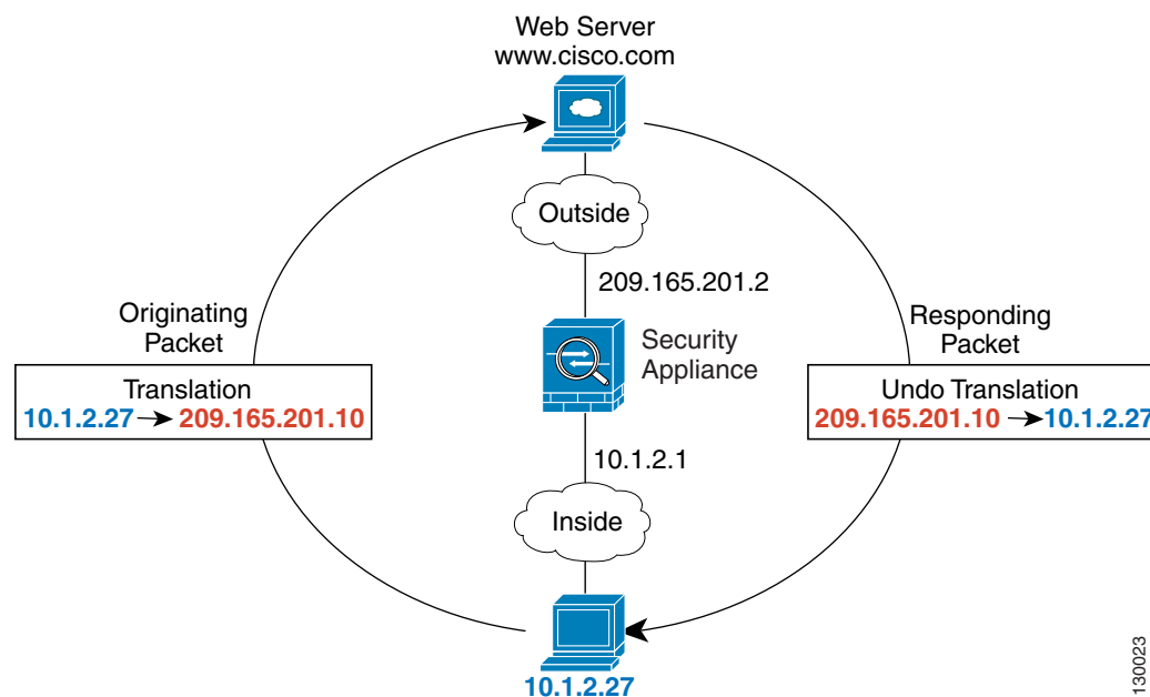
Figure 22-1 NAT Example: Routed Mode
