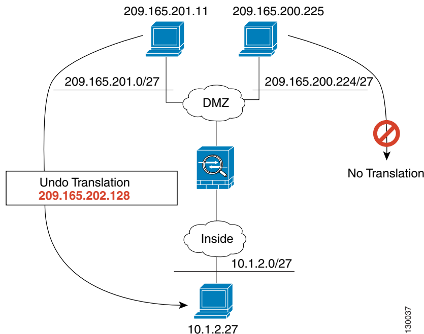
Figure 22-11 Policy Static NAT with Destination Address Translation
