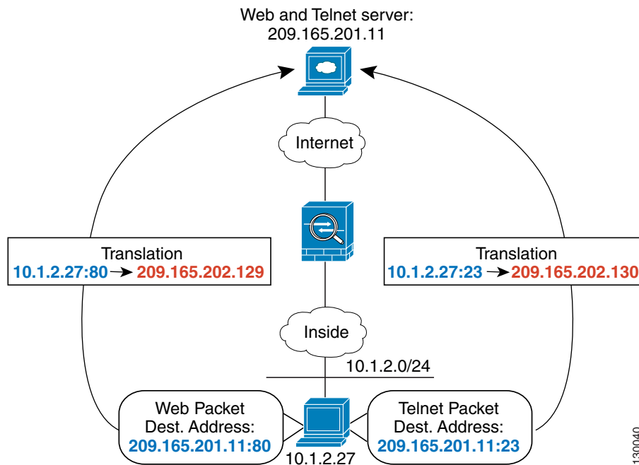
Figure 22-10 Policy NAT with Different Destination Ports
