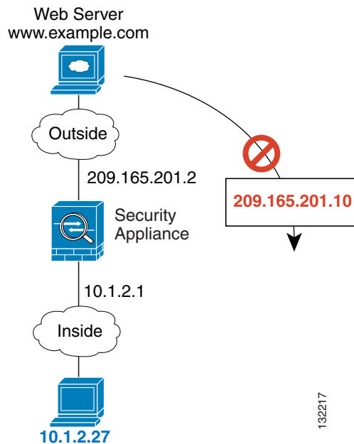
Figure 22-7 Remote Host Attempts to Initiate a Connection to a Mapped Address
