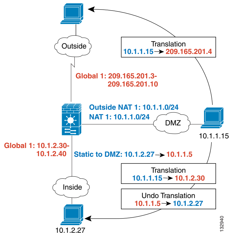
Figure 22-18 Outside NAT and Inside NAT Combined
