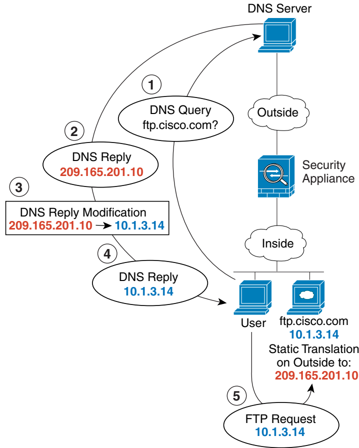
Figure 22-12 DNS Reply Modification
