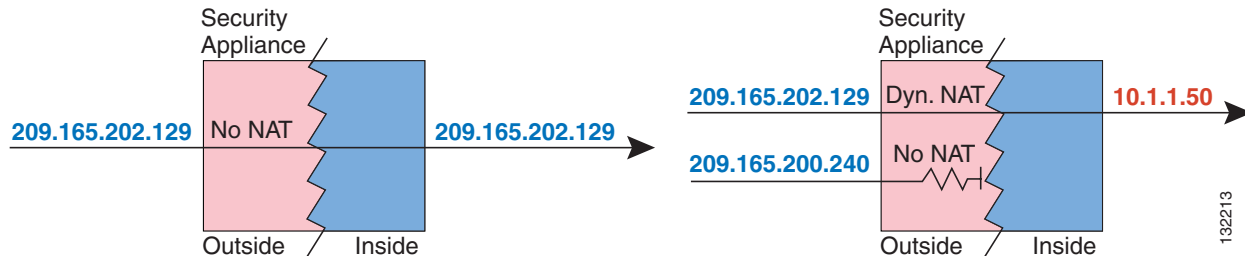
Figure 22-5 NAT Control and Inbound Traffic
