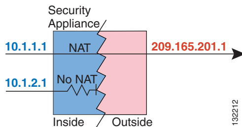
Figure 22-3 NAT Control and Outbound Traffic
