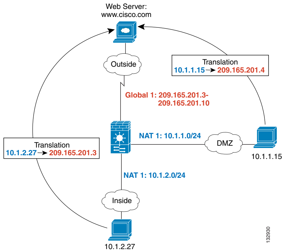
Figure 22-14 NAT Rules on Multiple Interfaces Using the Same Global Pool
