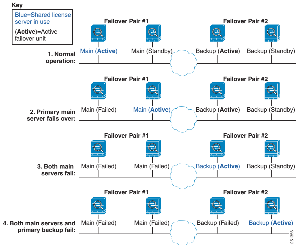
Figure 4-2 Failover and Shared License Servers
