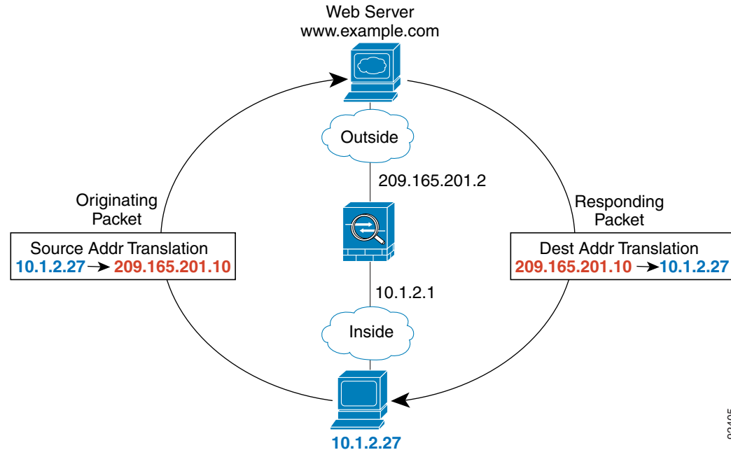
Figure 16-1 NAT Example
