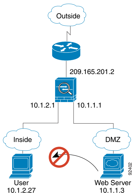
Figure 16-6 DMZ to Inside
