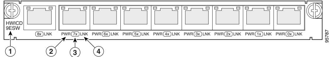
Figure 110 HWIC-D-9ESW Faceplate
