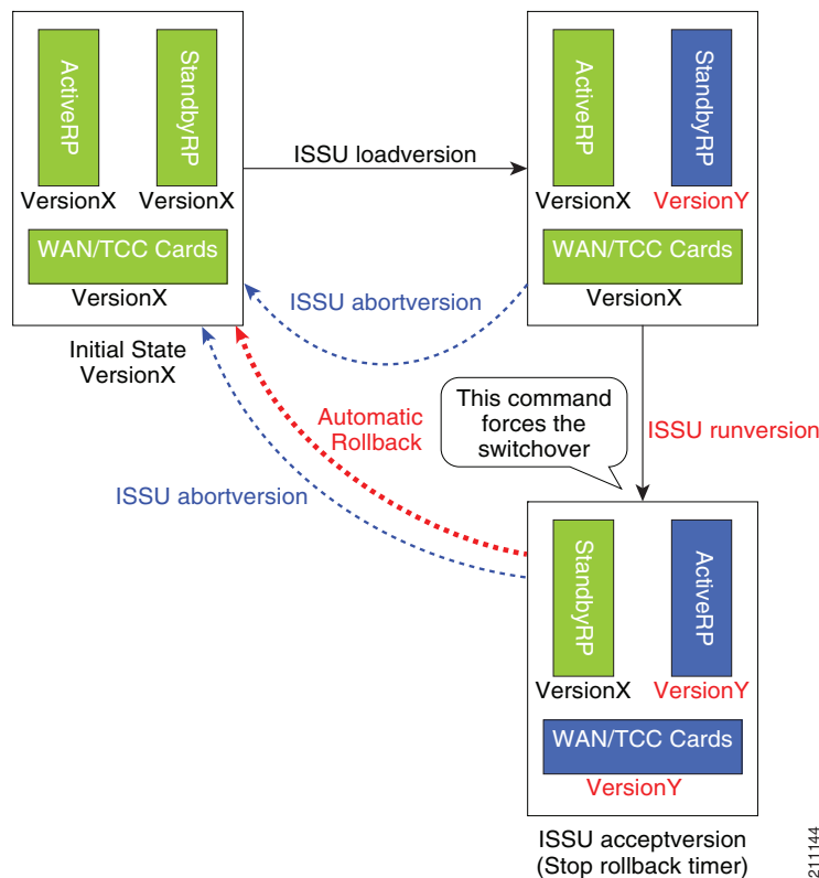
Figure 9 RP ISSU Process Stages With WAN Line Card MDR
