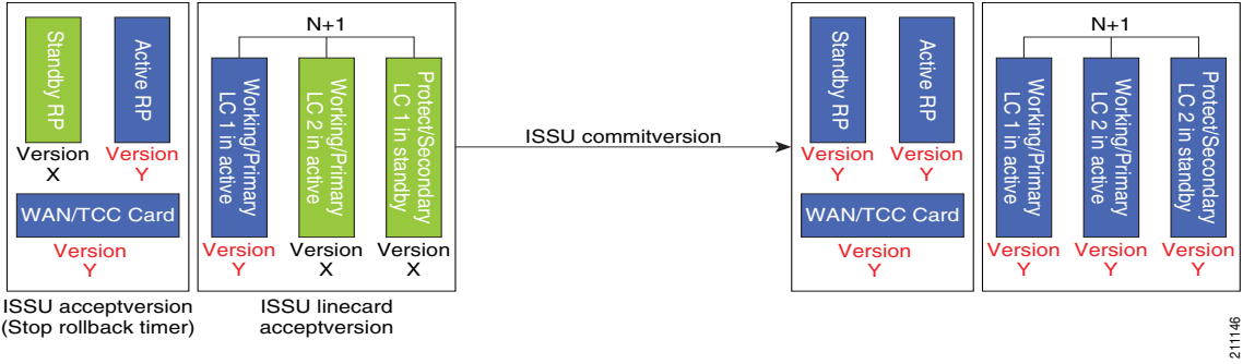
Figure 11 Combined RP and RLC ISSU Commit Version Stage
