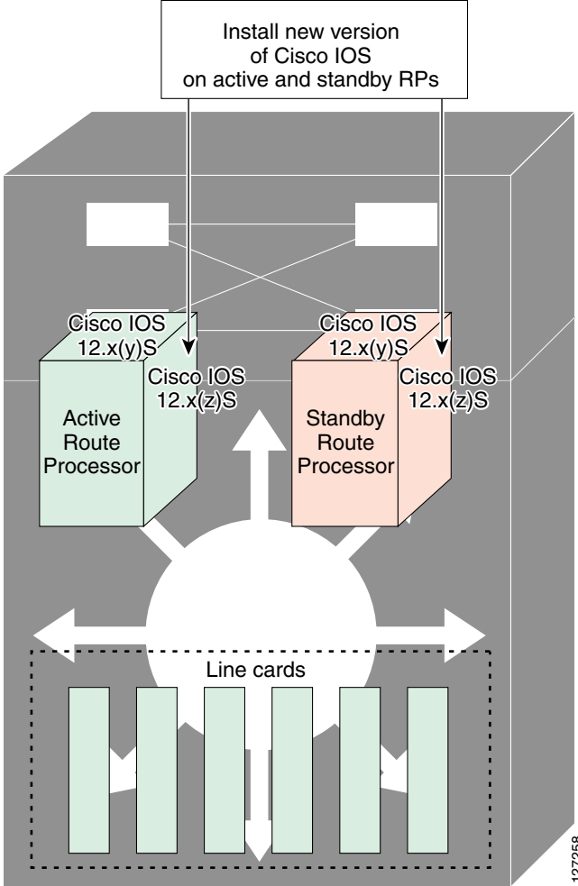
Figure 2 How to Load New Cisco IOS Software on Both RPs
