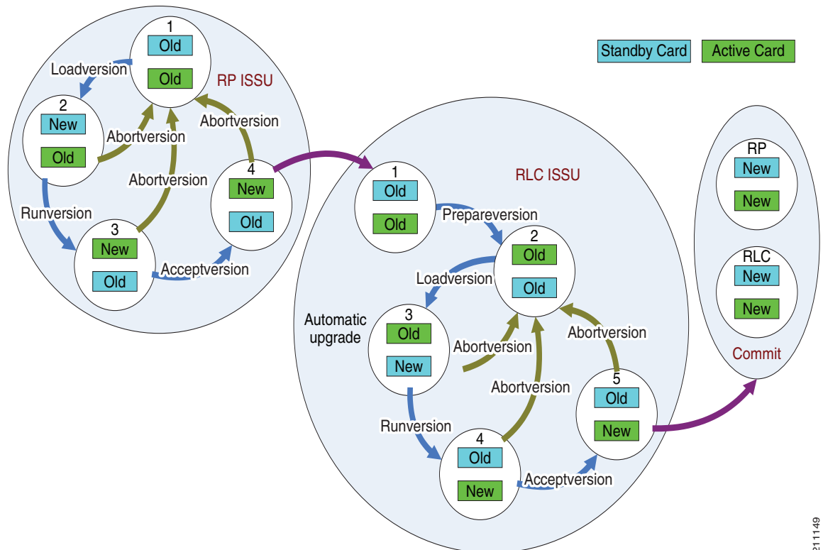
Figure 12 RP and RLC ISSU Process Summary View
