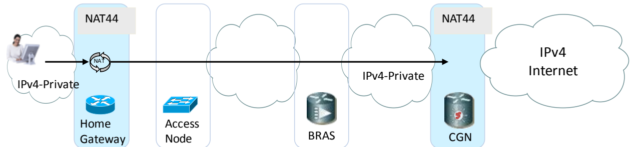
Network with Carrier-Grade NAT444
