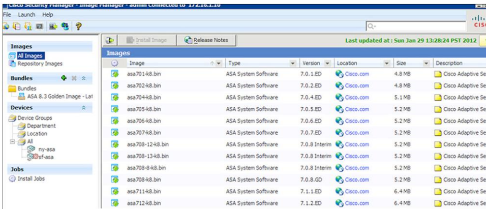
Figure 6. Software Image Upgrade Wizard
