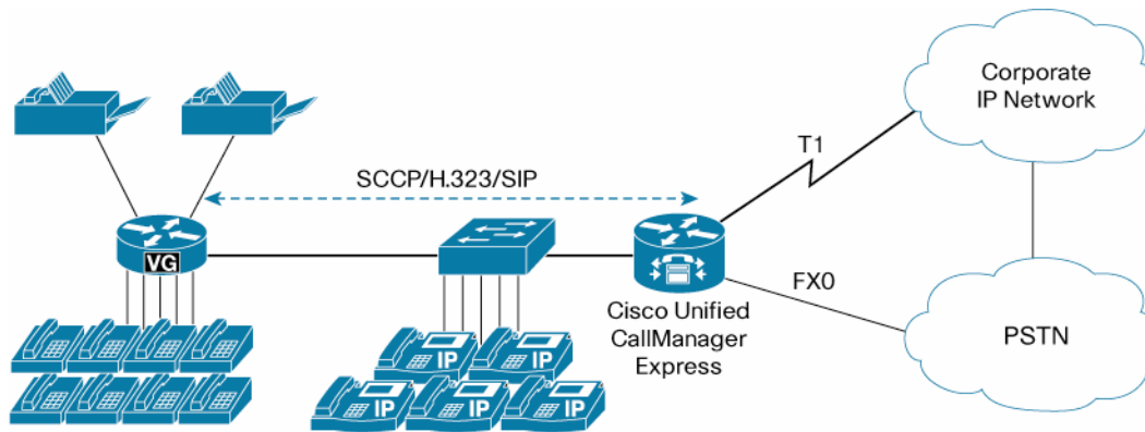
Figure 6. Cisco VG Integration with Cisco Unified Communications Manager Express
