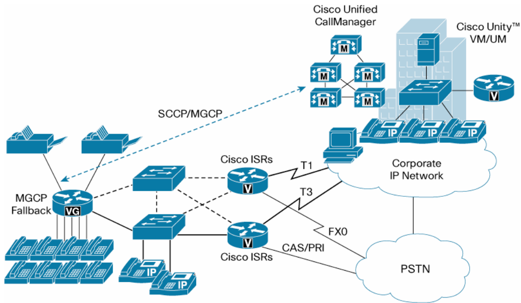
Figure 5. Cisco VG Integration with Cisco Unified Communications Manager
