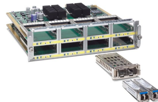
Figure 5 8-Port (2:1) 10 Gigabit Ethernet (X2) Half Card (Cisco TwinGig Support up to 16GE Ports)
