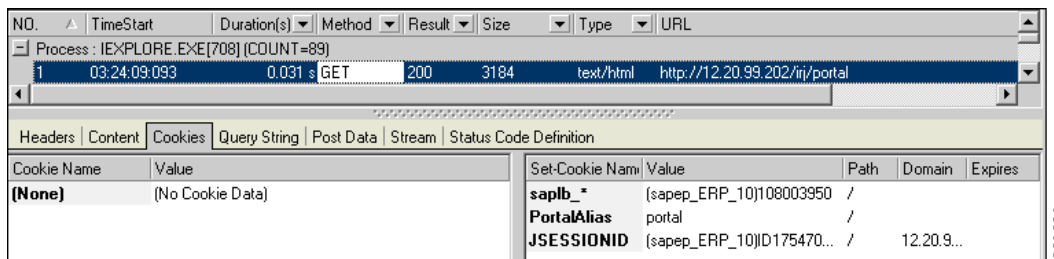
Figure 9 Cookie Analysis for HTTP Request #1
