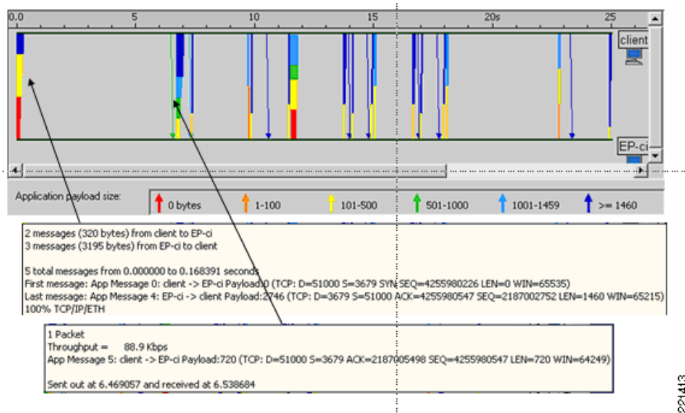
Figure 19 SAP ESS Transaction—Message Timeline
