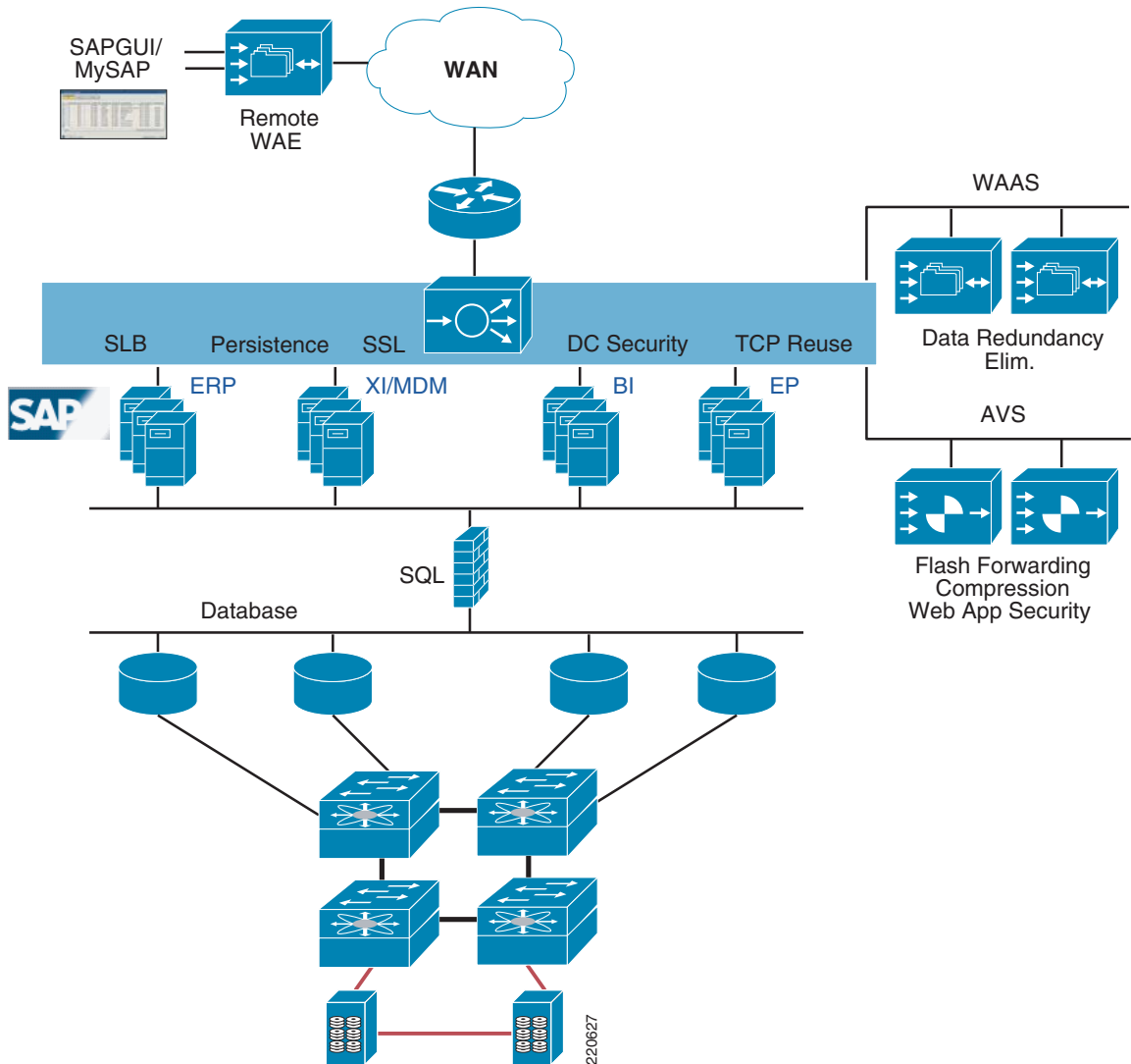
Figure 2 SAP Logical Design
