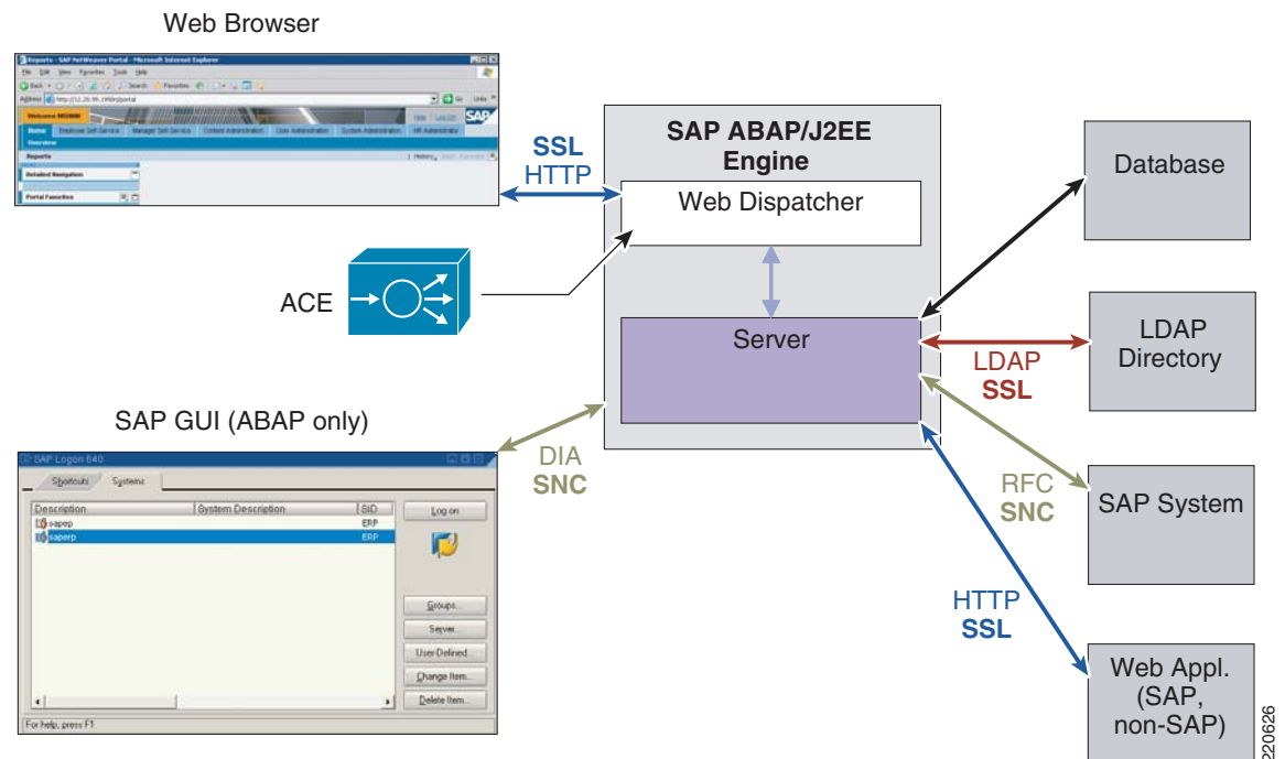
Figure 1 SAP Architecture
