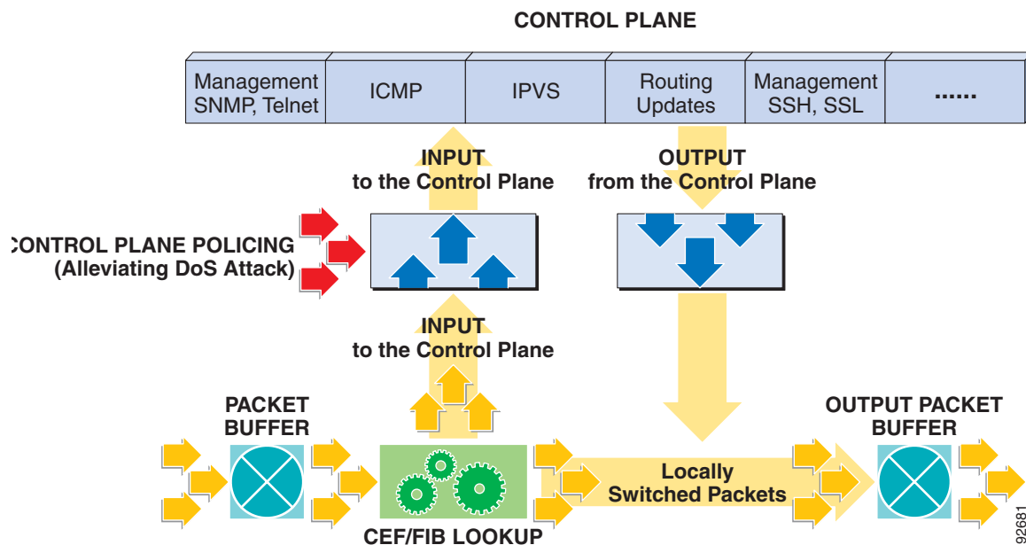
Figure 3 Centralized CoPP
