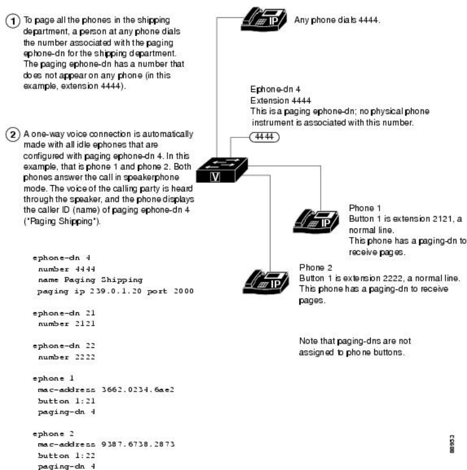
Figure 1: Paging Group
