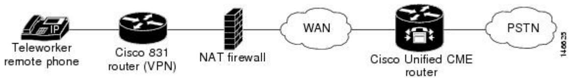
Figure 8: Remote Site IP Phones Using NAT
