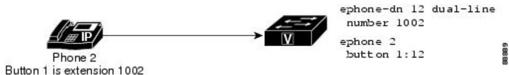
Figure 2: Dual-Line Directory Number
