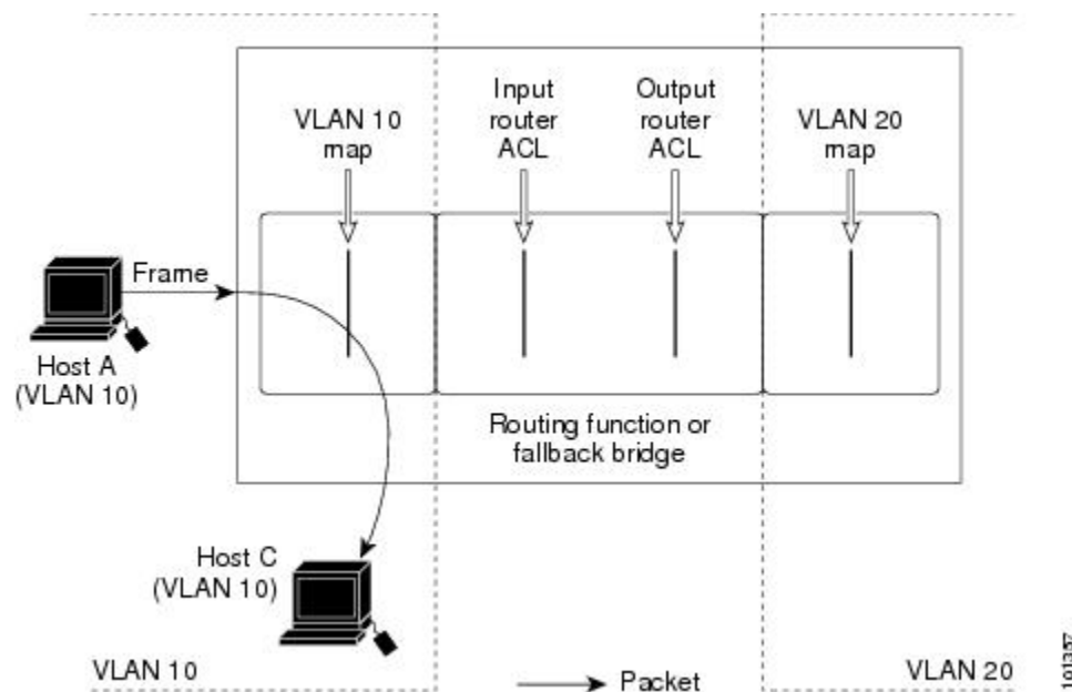
Figure 78: Applying ACLs on Switched Packets
