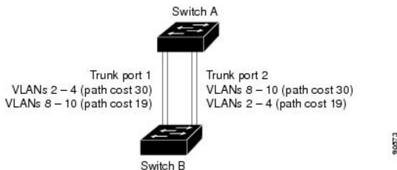
Figure 105: Load-Sharing Trunks with Traffic Distributed by Path Cost
