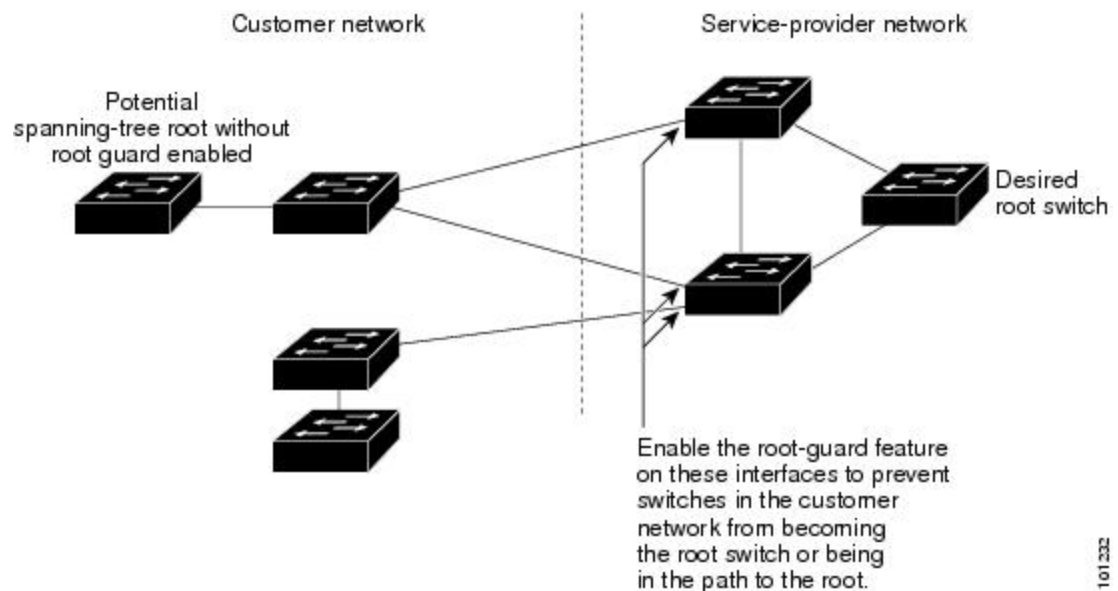
Figure 38: Root Guard in a Service-Provider Network
