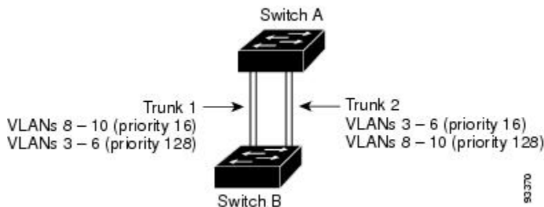
Figure 104: Load Sharing by Using STP Port Priorities
