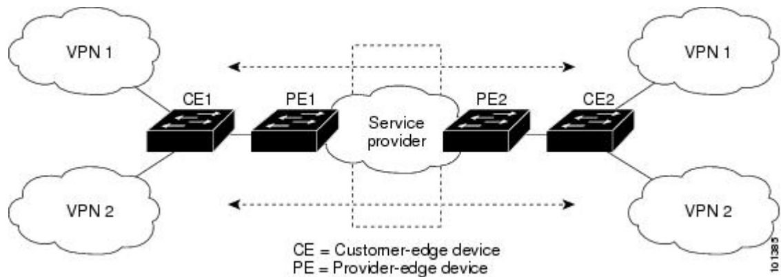
Figure 69: Switches Acting as Multiple Virtual CEs
