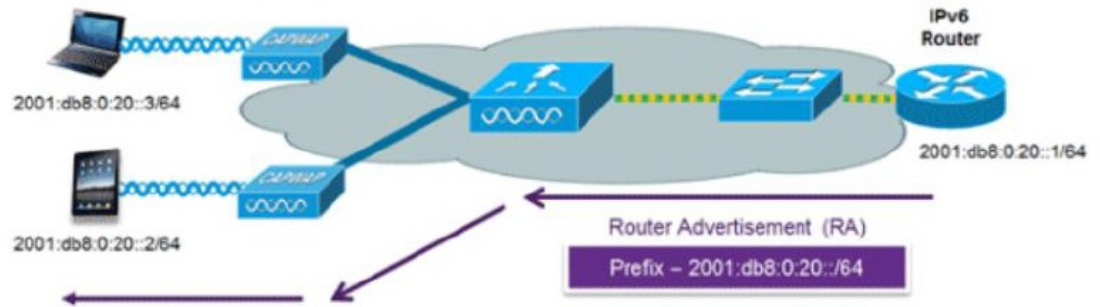
Figure 16: SLAAC Address Assignment
