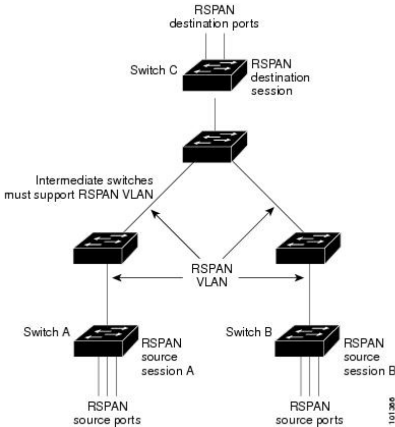
Figure 59: Example of RSPAN Configuration
