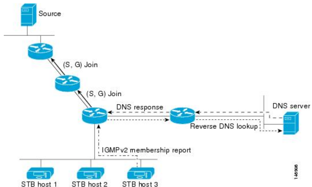
Figure 12: DNS-Based SSM Mapping
