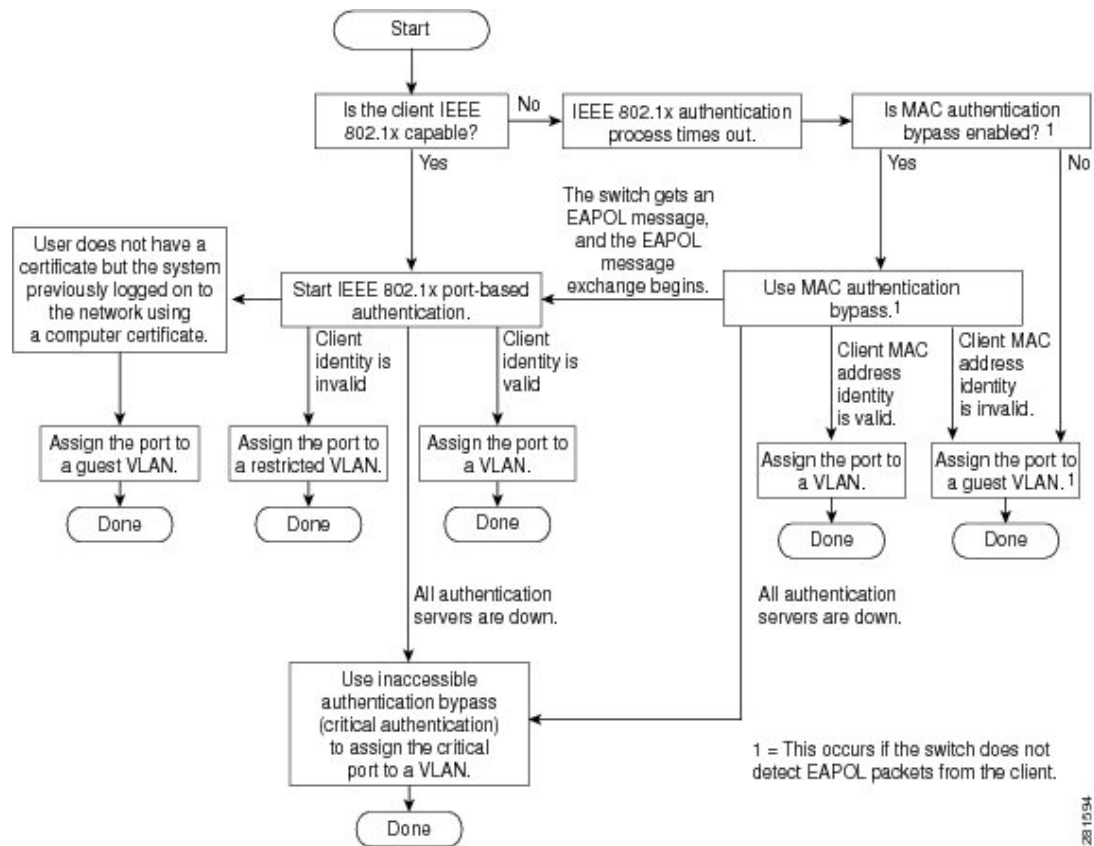
Figure 87: Authentication Flowchart
