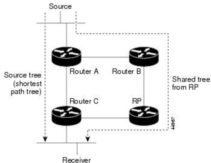
Figure 10: Shared Tree and Source Tree (Shortest-Path Tree)
