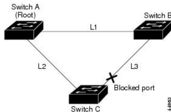
Figure 35: BackboneFast Example Before Indirect Link Failure
