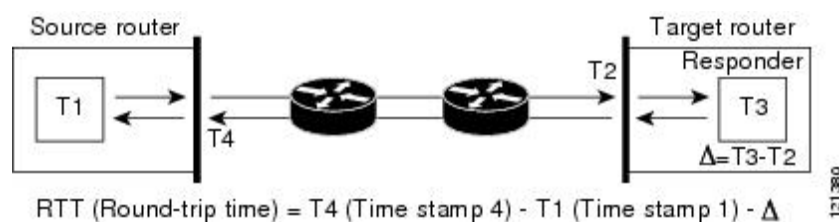
Figure 56: Cisco IOS IP SLA Responder Time Stamping
