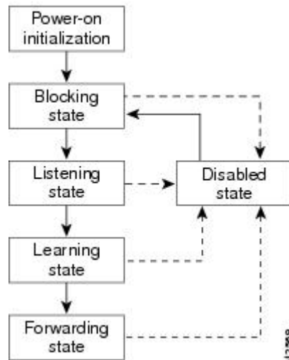
Figure 22: Spanning-Tree Interface States
