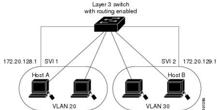
Figure 2: Connecting VLANs with the Switch
