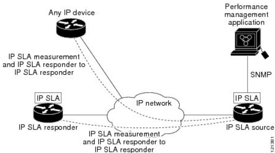
Figure 55: Cisco IOS IP SLAs Operation
