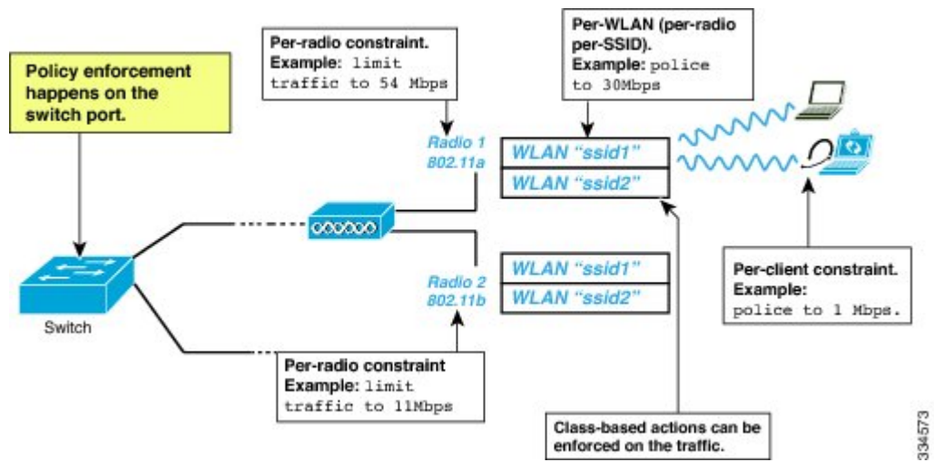
Figure 60: Hierarchical QoS
