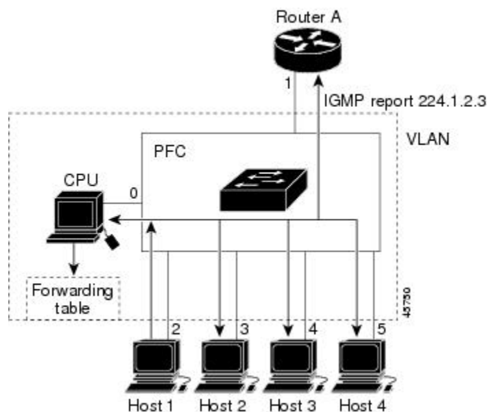
Figure 6: Initial IGMP Join Message
