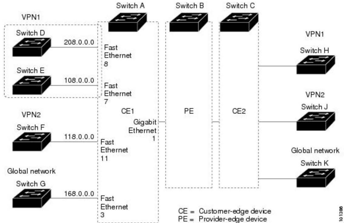
Figure 70: Multi-VRF CE Configuration Example
