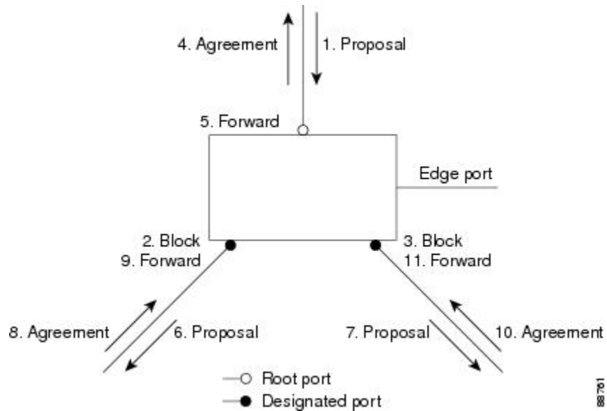
Figure 29: Sequence of Events During Rapid Convergence
