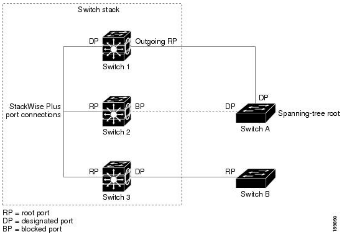
Figure 21: Spanning-Tree Port States in a Switch Stack
