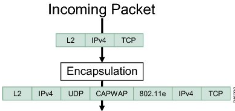
Figure 61: Wireless Packet Path in the Egress Direction during First Pass
