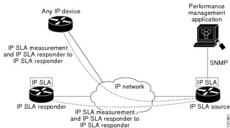
Figure 54: Cisco IOS IP SLAs Operation
