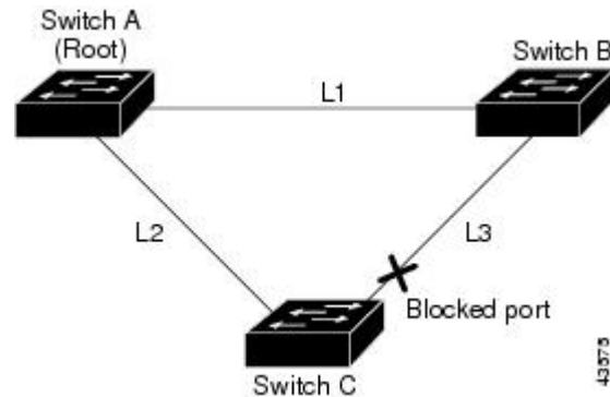
Figure 32: UplinkFast Example Before Direct Link Failure
