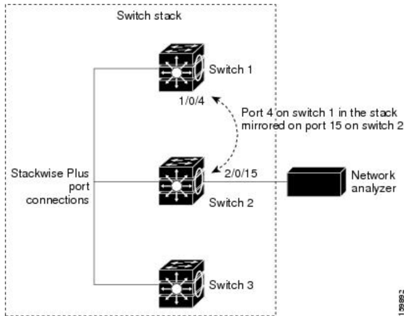
Figure 58: Example of Local SPAN Configuration on a Device Stack
