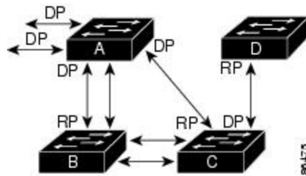
Figure 23: Spanning-Tree Topology
