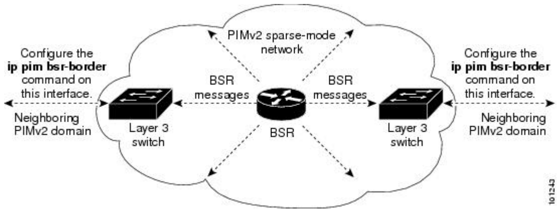
Figure 11: Constraining PIMv2 BSR Messages
