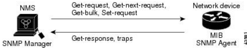
Figure 53: SNMP Network
