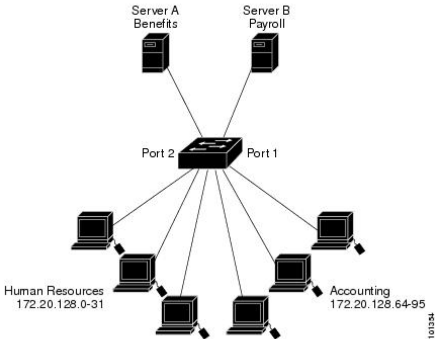
Figure 75: Using Router ACLs to Control Traffic
