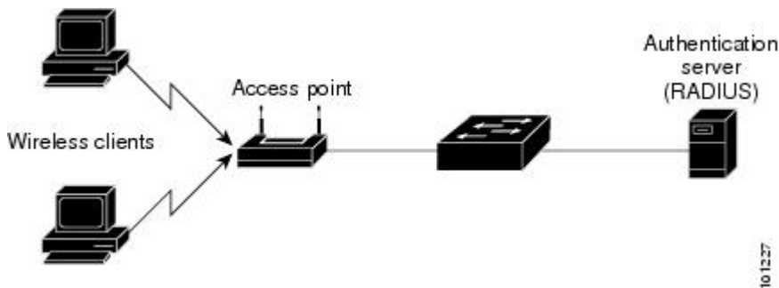
Figure 90: Multiple Host Mode Example
