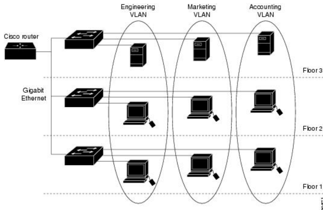
Figure 103: VLANs as Logically Defined Networks
