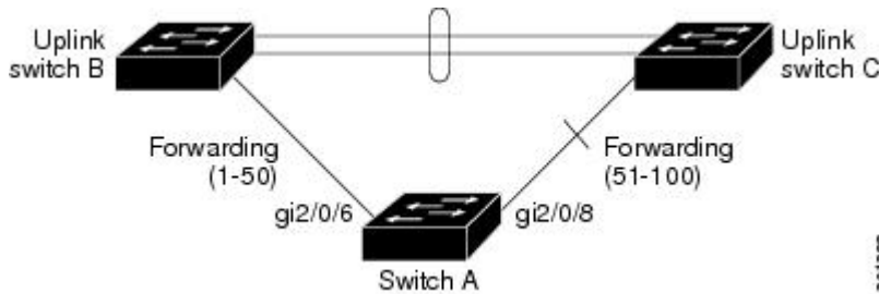
Figure 45: VLAN Flex Links Load-Balancing Configuration Example
