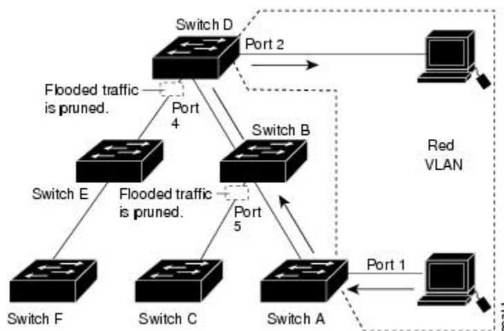
Figure 102: Optimized Flooded Traffic VTP Pruning
