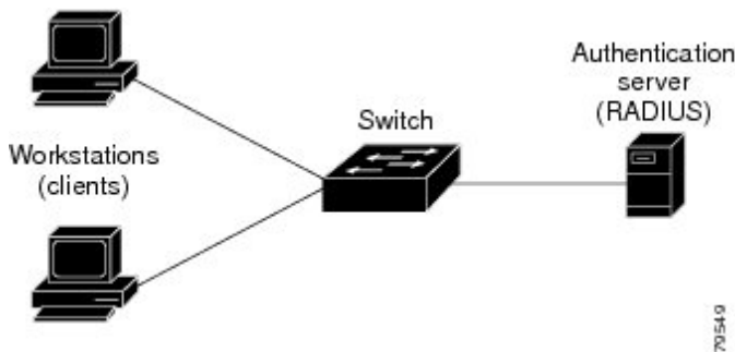
Figure 92: Web-Based Authentication Device Roles
