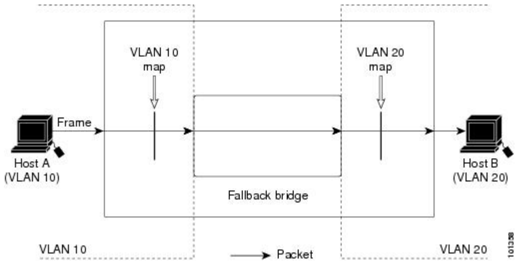
Figure 79: Applying ACLs on Bridged Packets
