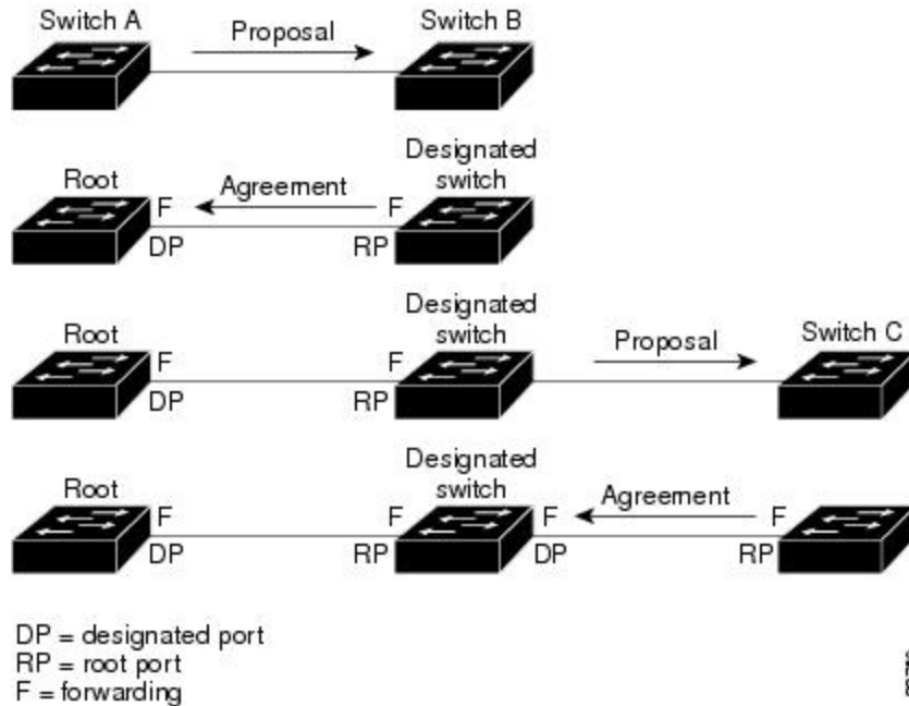
Figure 28: Proposal and Agreement Handshaking for Rapid Convergence
