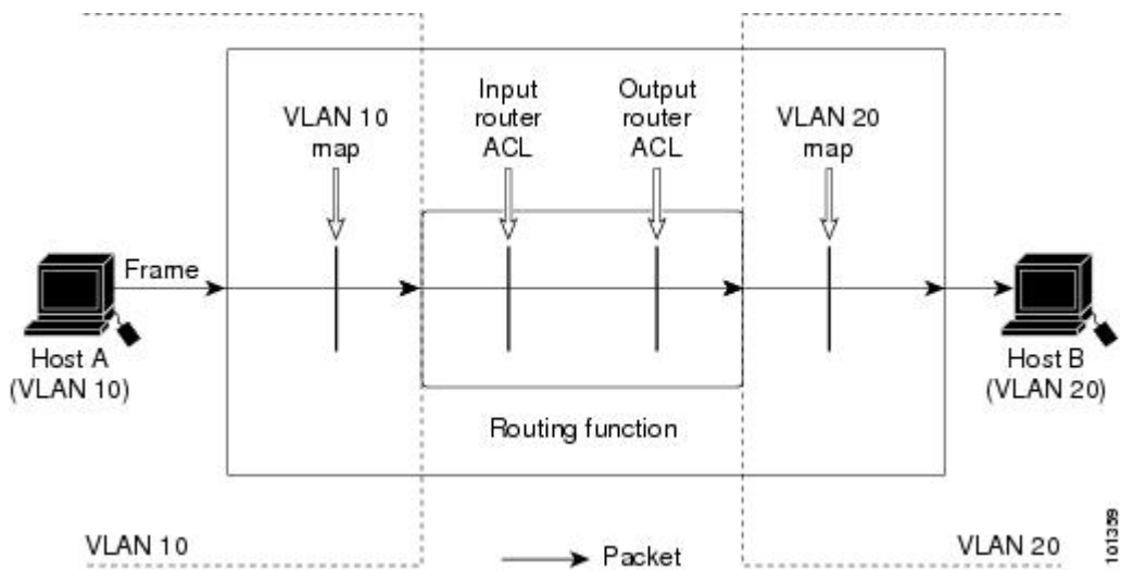
Figure 80: Applying ACLs on Routed Packets
