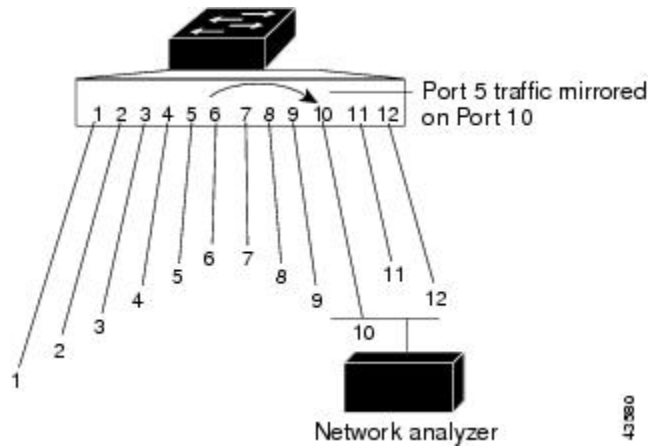
Figure 57: Example of Local SPAN Configuration on a Single Device
