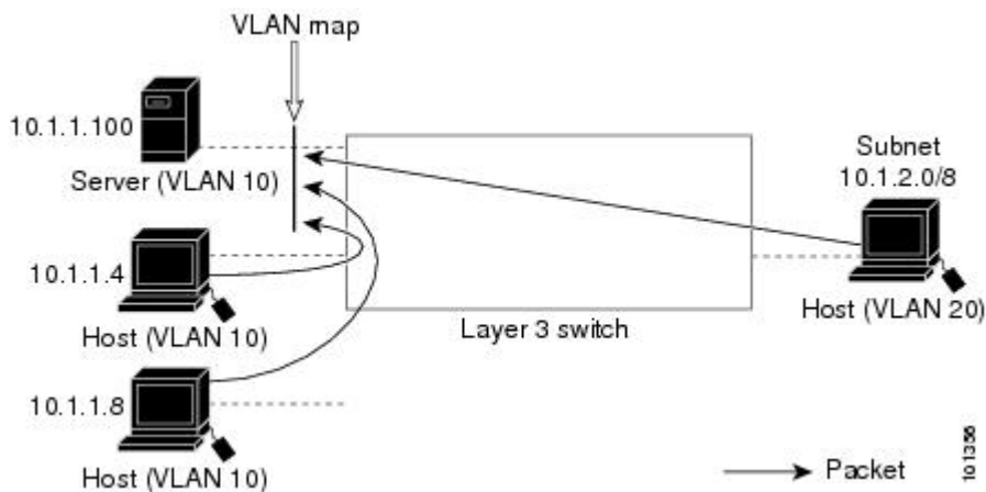
Figure 77: Restricting Access to a Server on Another VLAN
