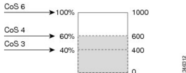
Figure 63: WTD and Queue Operation
