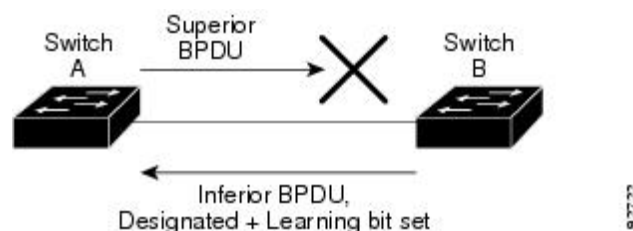
Figure 27: Detecting Unidirectional Link Failure
