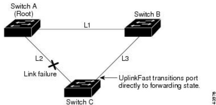
Figure 33: UplinkFast Example After Direct Link Failure
