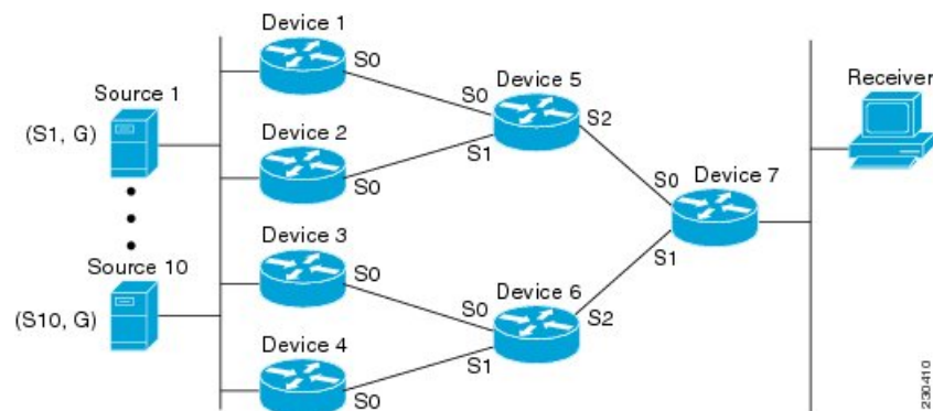
Figure 34: Polarization Topology
