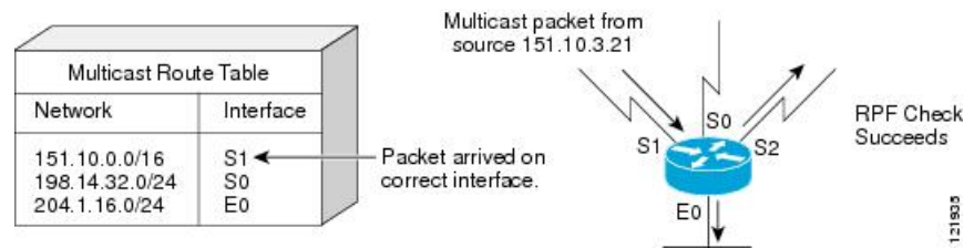
Figure 25: RPF Check Succeeds
