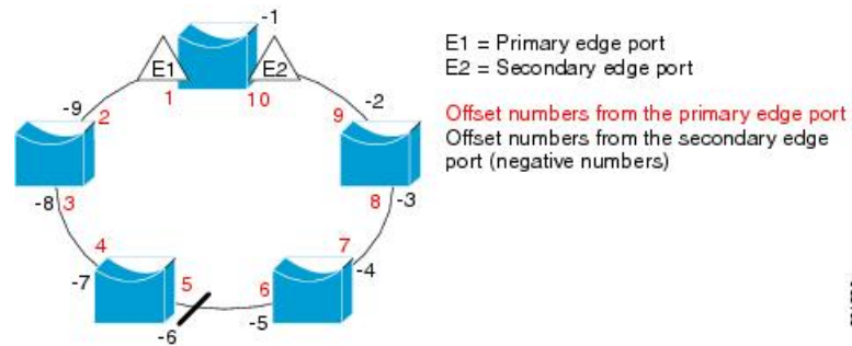
Figure 64: Neighbor Offset Numbers in a Segment
