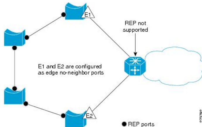
Figure 63: Edge No-Neighbor Ports
