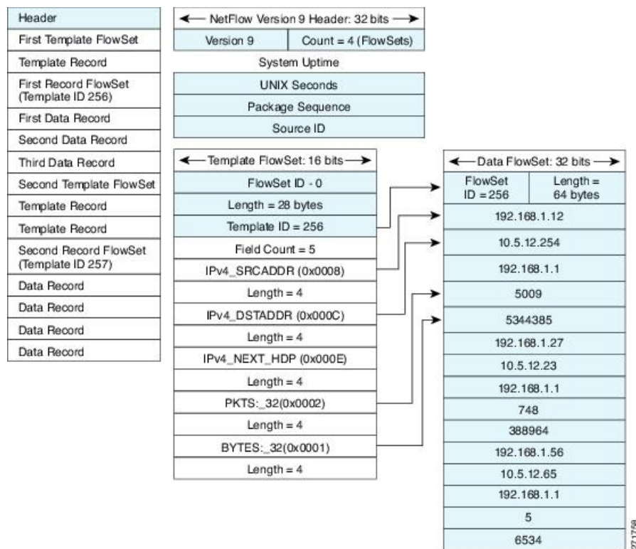
Figure 81: Detailed Example of the NetFlow Version 9 Export Format
