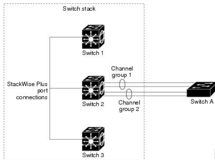
Figure 57: Single-Switch EtherChannel
