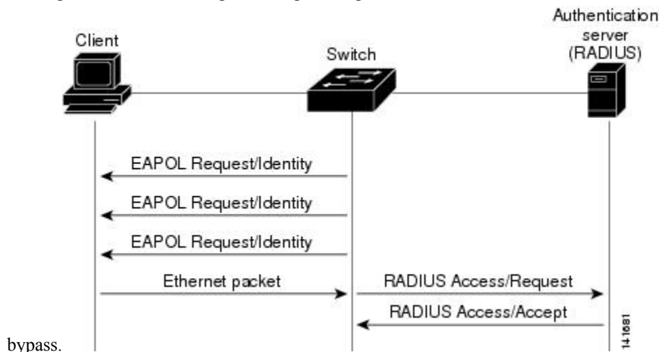
Figure 117: Message Exchange During MAC Authentication Bypass
