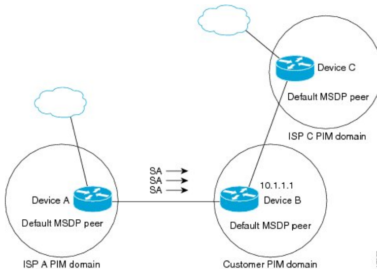
Figure 28: Default MSDP Peer Scenario
