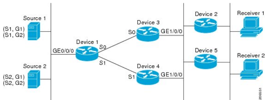
Figure 36: ECMP Multicast Load Splitting and the PIM Assert Process in PIM-SM and PIM-SSM
