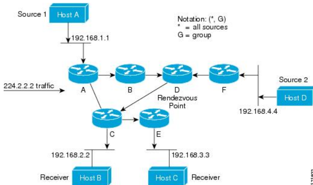
Figure 22: Shared Tree
