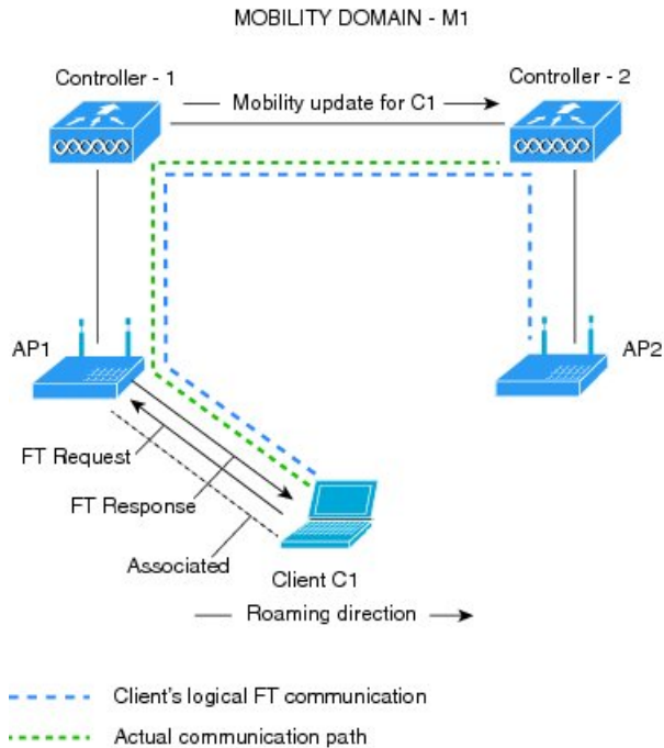
Figure 136: Message Exchanges when Over the DS client roaming is configured
