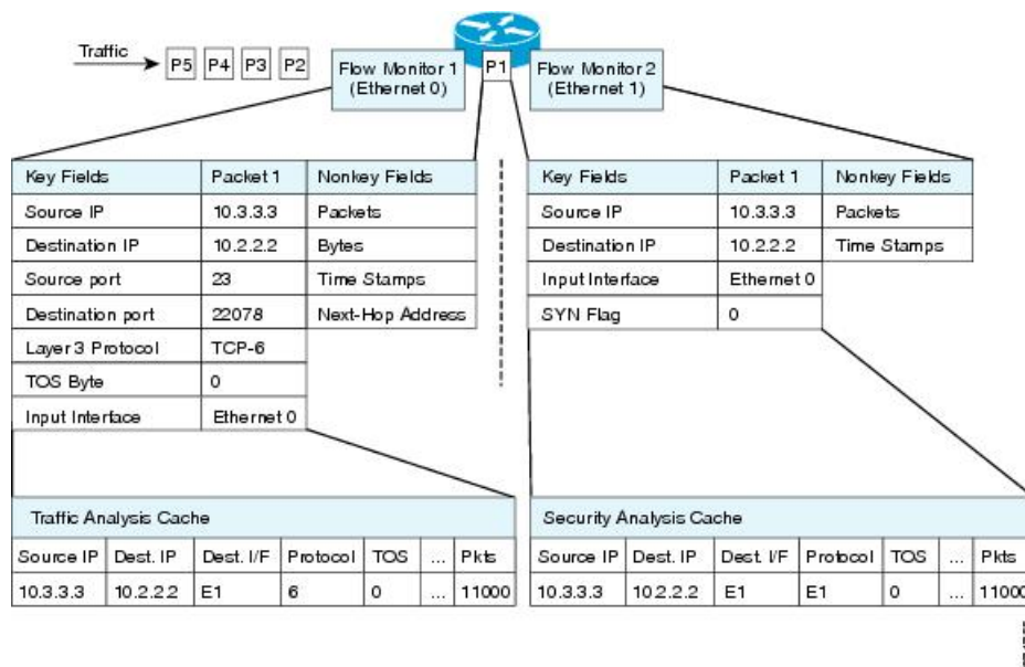
Figure 82: Example of Using Two Flow Monitors to Analyze the Same Traffic
