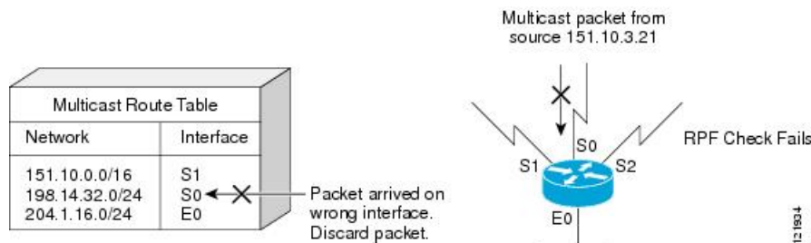
Figure 24: RPF Check Fails
