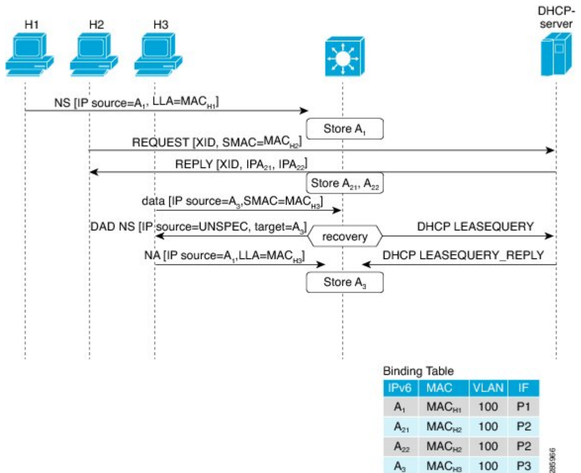
Figure 29: IPv6 Address Glean
