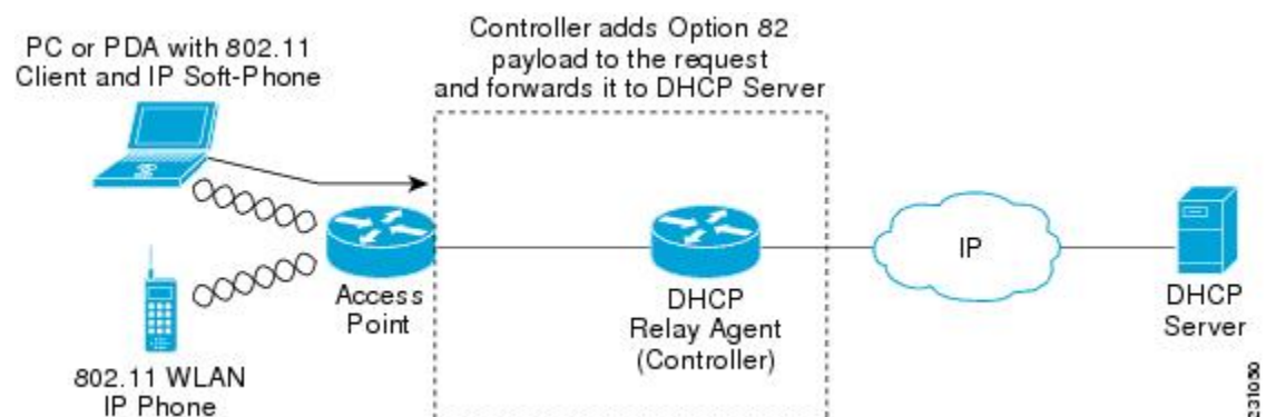
Figure 134: DHCP Option 82
