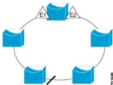
Figure 62: REP Ring Segment
