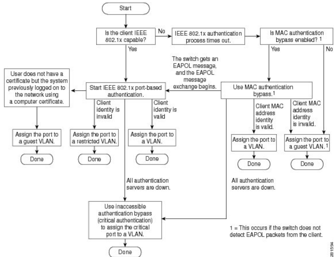
Figure 115: Authentication Flowchart
