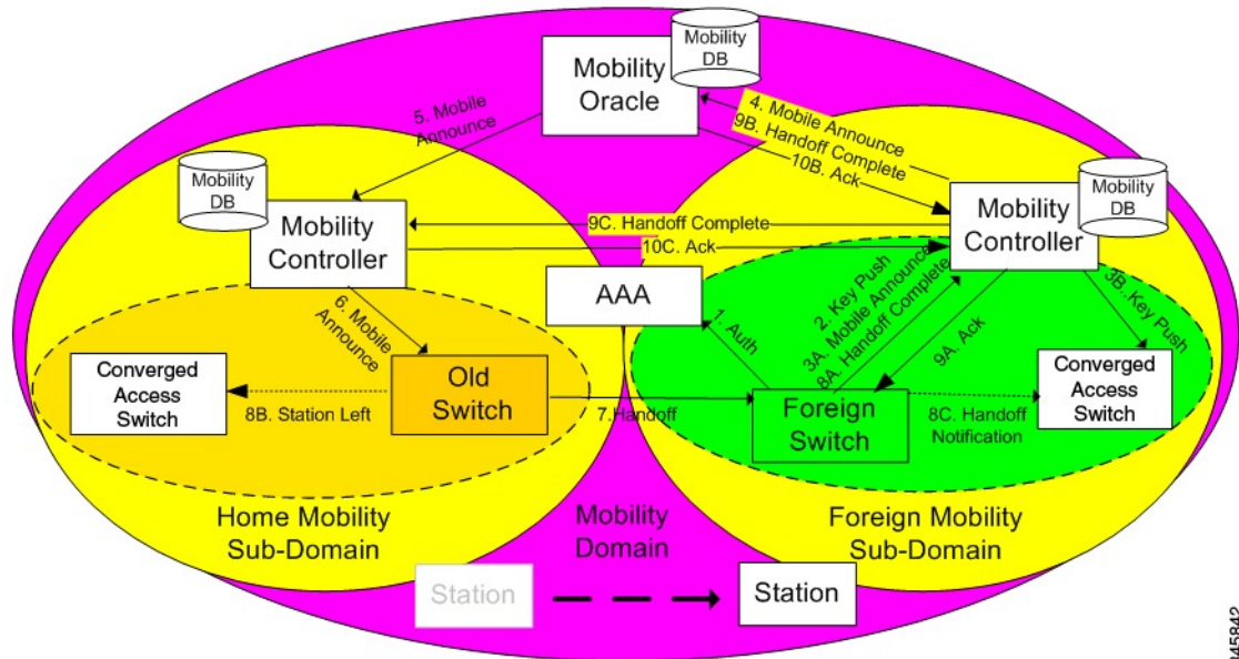
Figure 68: Inter Sub Domain Handoff
