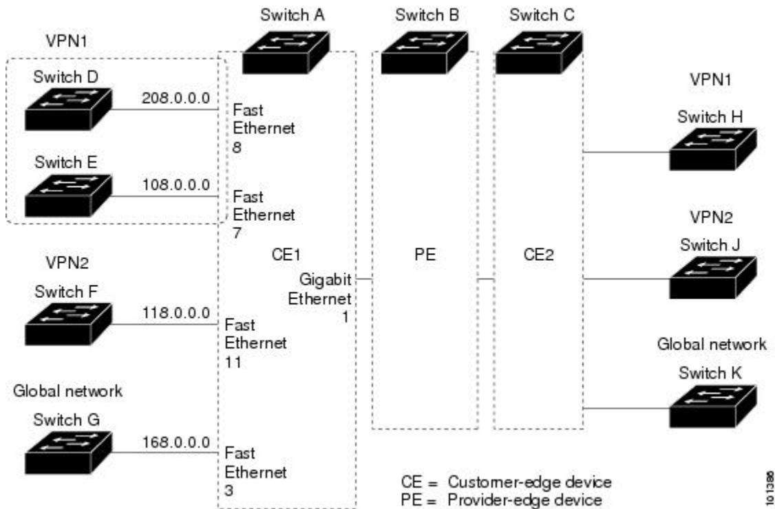
Figure 95: Multi-VRF CE Configuration Example
