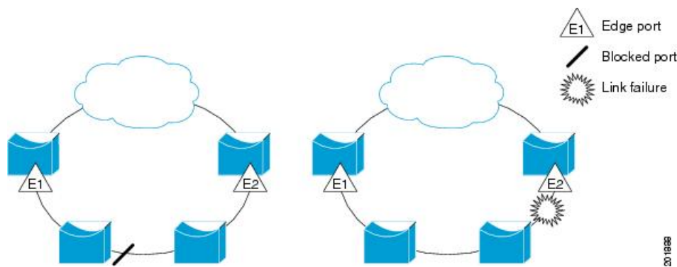
Figure 61: REP Open Segment
