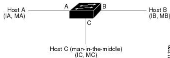
Figure 111: ARP Cache Poisoning
