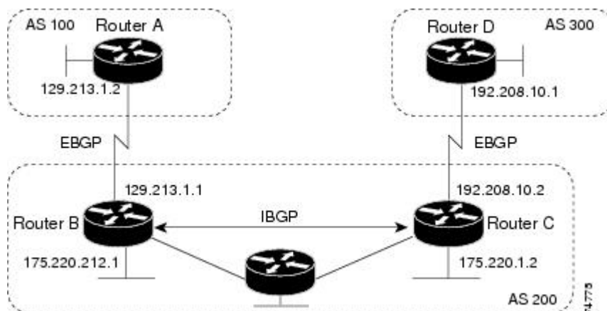
Figure 92: EBGP, IBGP, and Multiple Autonomous Systems
