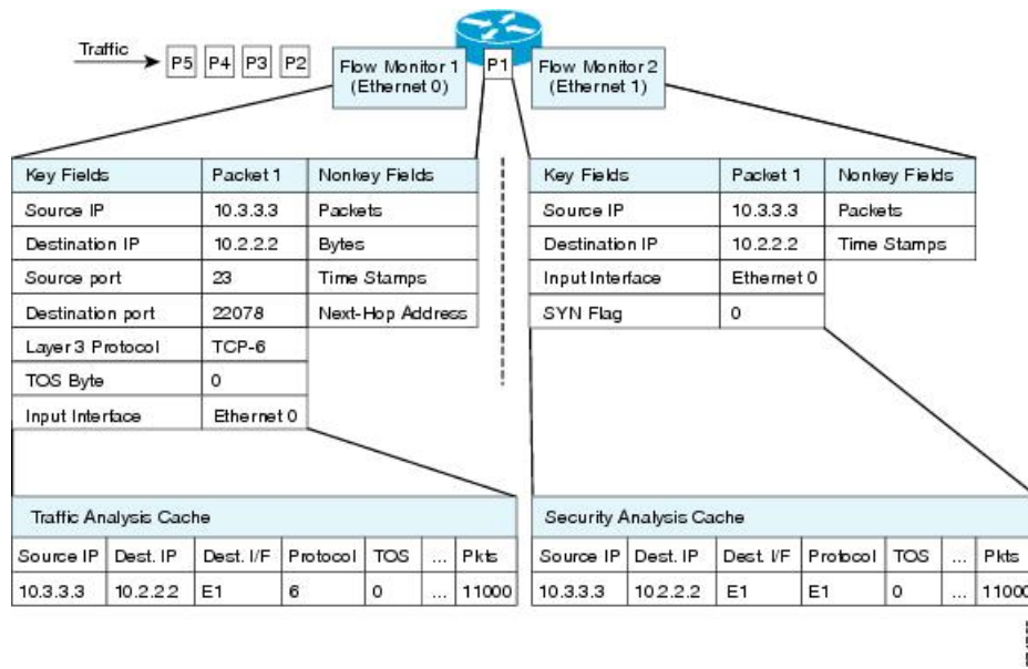
Figure 76: Example of Using Two Flow Monitors to Analyze the Same Traffic
