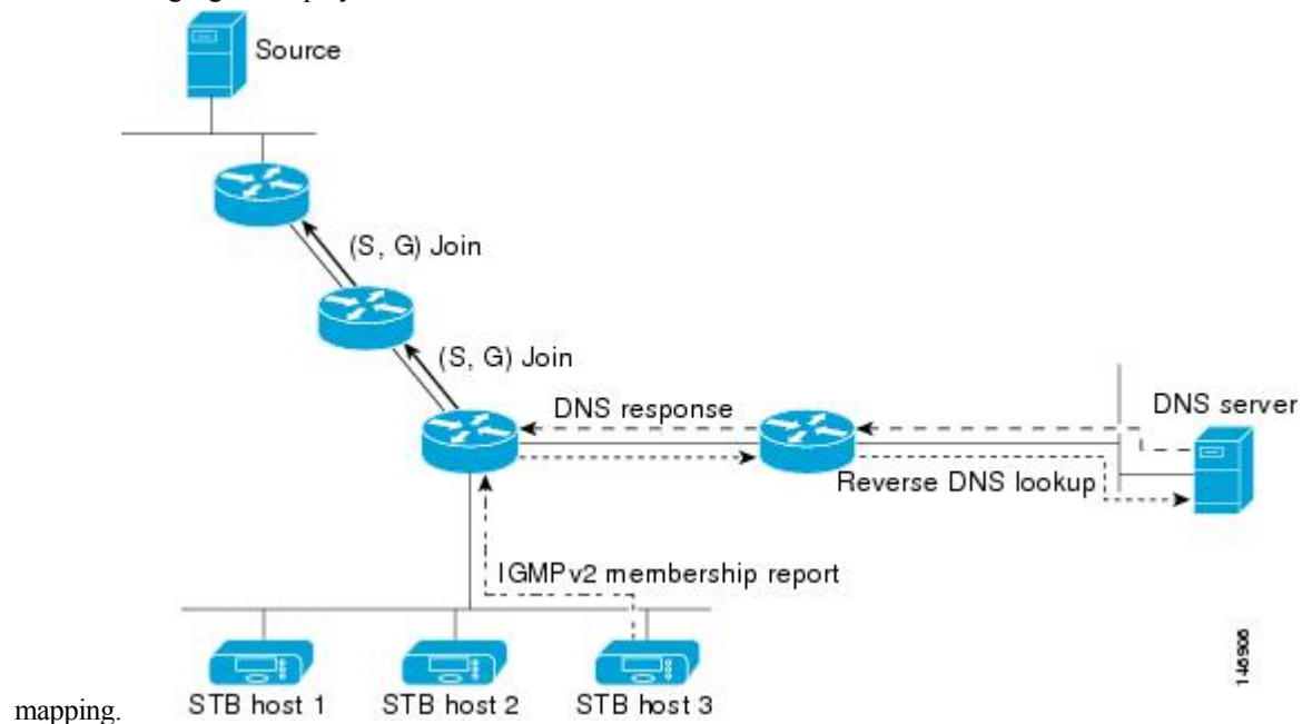
Figure 29: DNS-Based SSM Mapping
