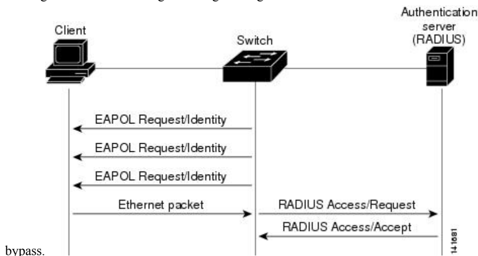
Figure 109: Message Exchange During MAC Authentication Bypass
