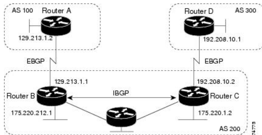
Figure 87: EBGP, IBGP, and Multiple Autonomous Systems
