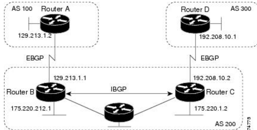
Figure 86: EBGP, IBGP, and Multiple Autonomous Systems
