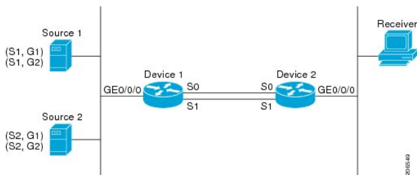
Figure 32: Default Behavior for IP Multicast When Multiple Equal-Cost Paths Exist
