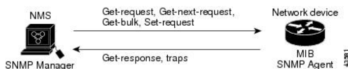
Figure 66: SNMP Network
