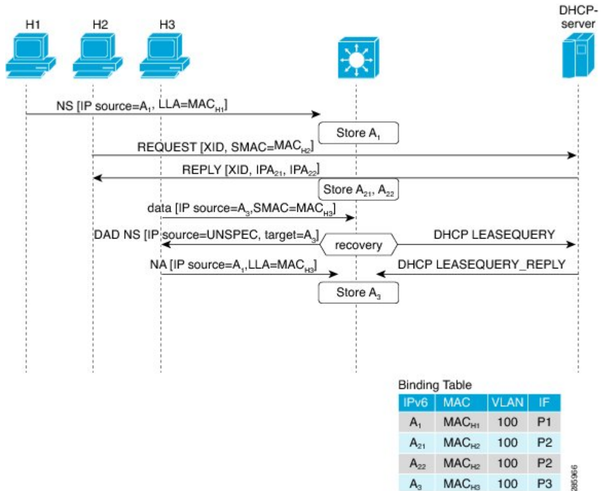
Figure 28: IPv6 Address Glean
