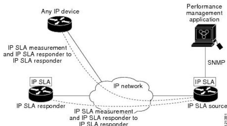
Figure 68: Cisco IOS IP SLAs Operation
