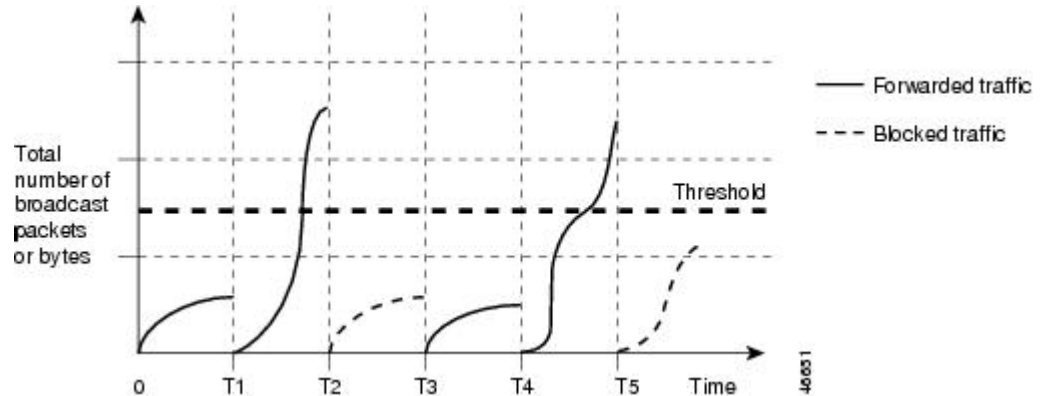
Figure 116: Broadcast Storm Control Example
