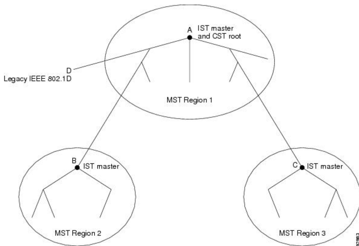
Figure 41: MST Regions, CIST Masters, and CST Root
