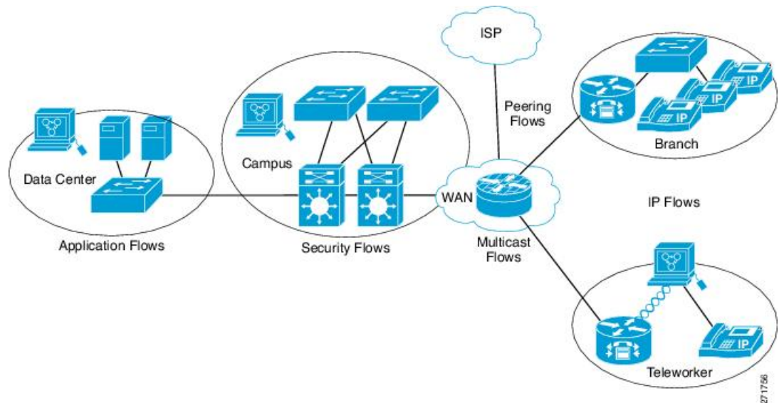
Figure 77: Complex Example of Using Multiple Types of Flow Monitors with Custom Records
