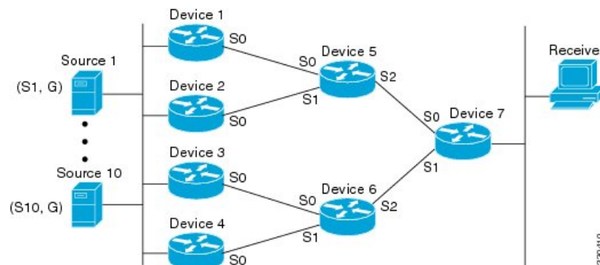
Figure 33: Polarization Topology
