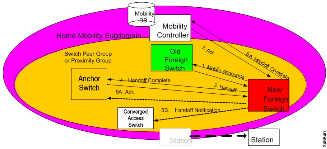
Figure 61: Intra Switch Peer Group Handoff
