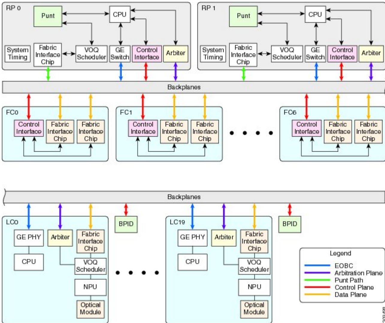
Figure 5: Major System Components and Interconnections in the Cisco ASR 9922 Router
