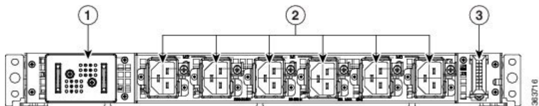
Figure 20: Version 3 Rear Panel
