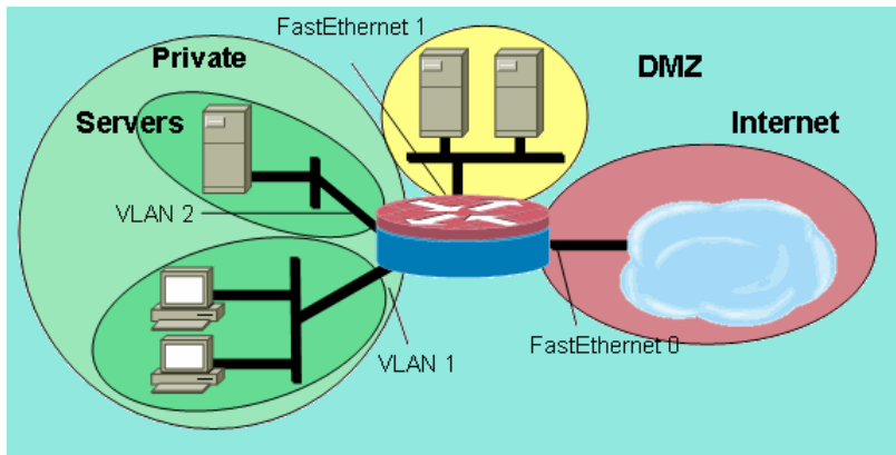
Figure 2: Zone Topology Detail
