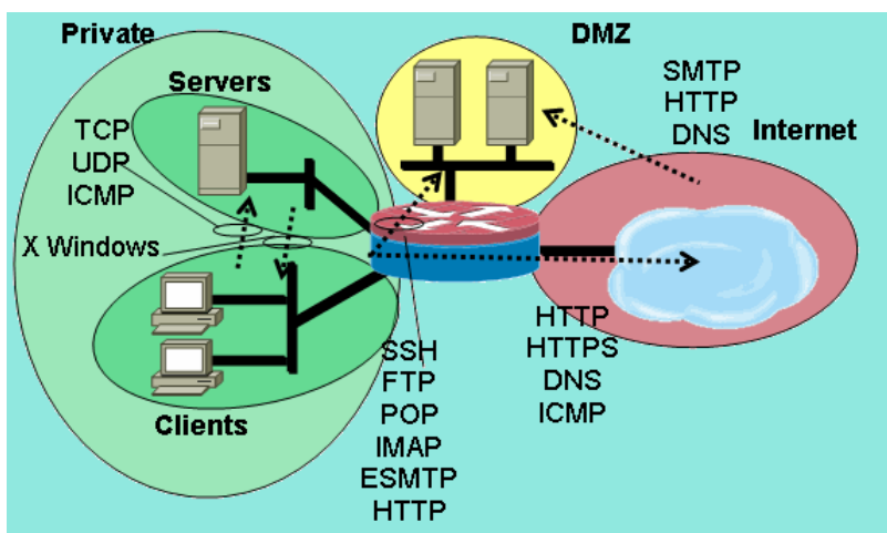
Figure 3: Zone-Pair service permissions to be applied in the configuration example
