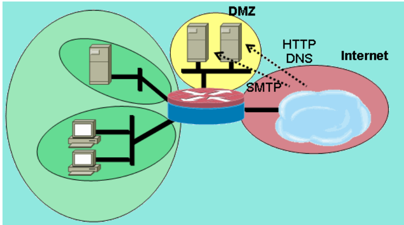
Figure 6: Service inspection from Internet zone to DMZ zone
