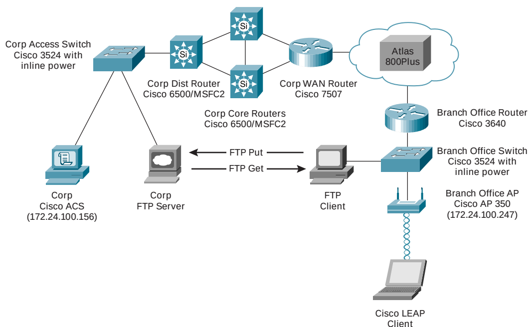
Figure 3 Testbed Setup
