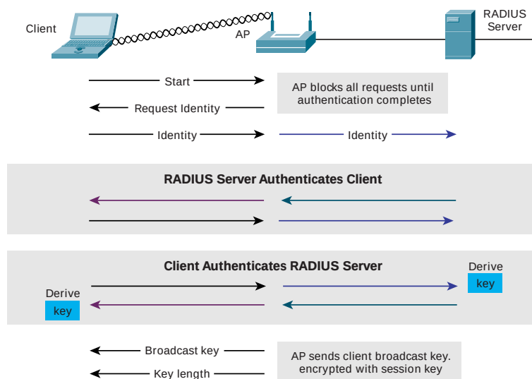
Figure 2 Authentication Process with 802.1x
