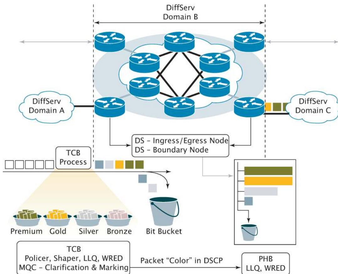
Figure 4. DiffServ Architecture
