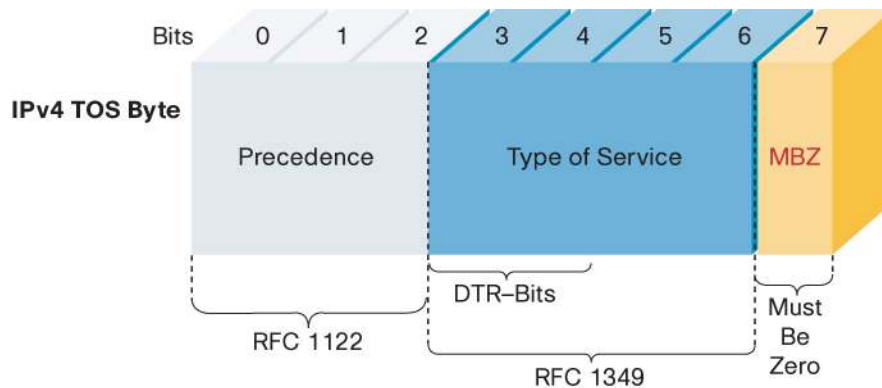
Figure 2. The Original IPv4 ToS Byte
