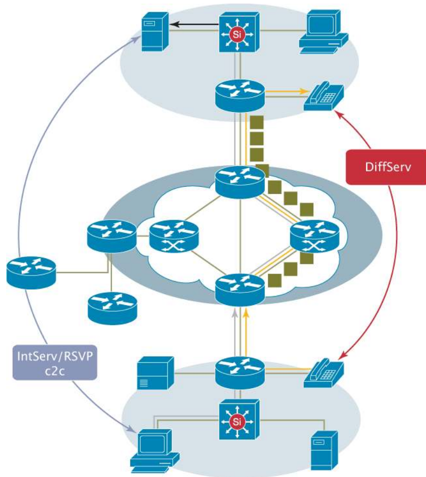
Figure 6. IntServ Over DiffServ Today
