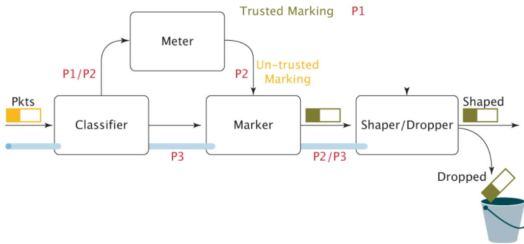
Figure 5. DiffServ Traffic Conditioner Block (TCB)
