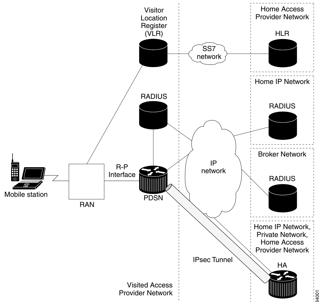
Figure 7 IS-835-B IPSec Network
