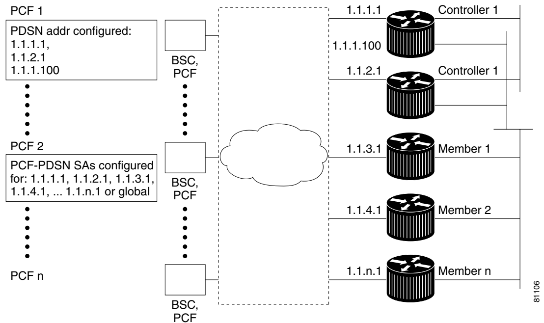
Figure 8 PDSN Controller -Member Architecture for 7200
