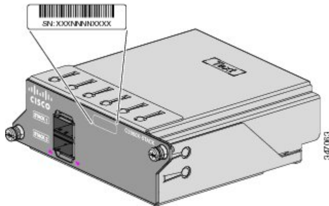
Figure 2: Serial Number Location for the FlexStack-Plus Module
