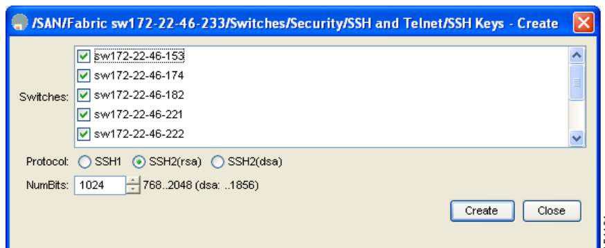
Figure 39-11 Create SSH and Telnet Dialog Box
