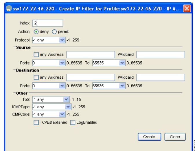
Figure 42-5 Create IP Filter Dialog Box
