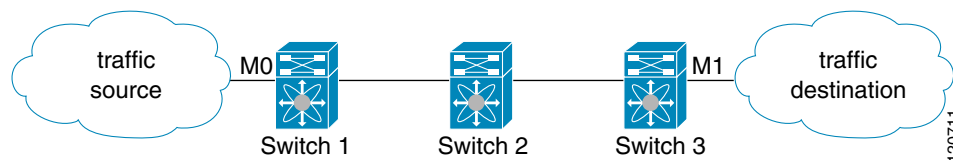
Figure 42-6 Denying Traffic on the Inbound Interface
