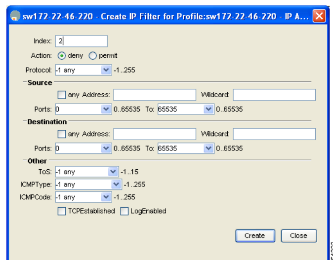
Figure 40-5 Create IP Filter Dialog Box
