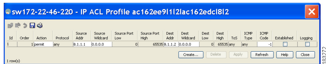
Figure 40-4 IP ACL Profile Dialog Box
