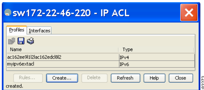
Figure 40-2 IP ACL Dialog Box
