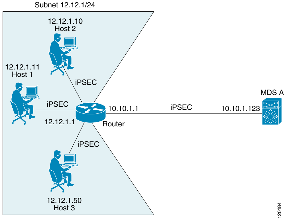
Figure 37-9 iSCSI with End-to-End IPsec
