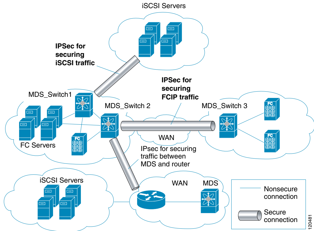
Figure 37-1 FCIP and iSCSI Scenarios Using MPS-14/2 Modules
