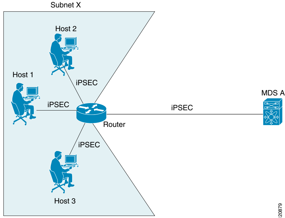
Figure 37-7 iSCSI with End-to-End IPsec Using the auto-peer Option
