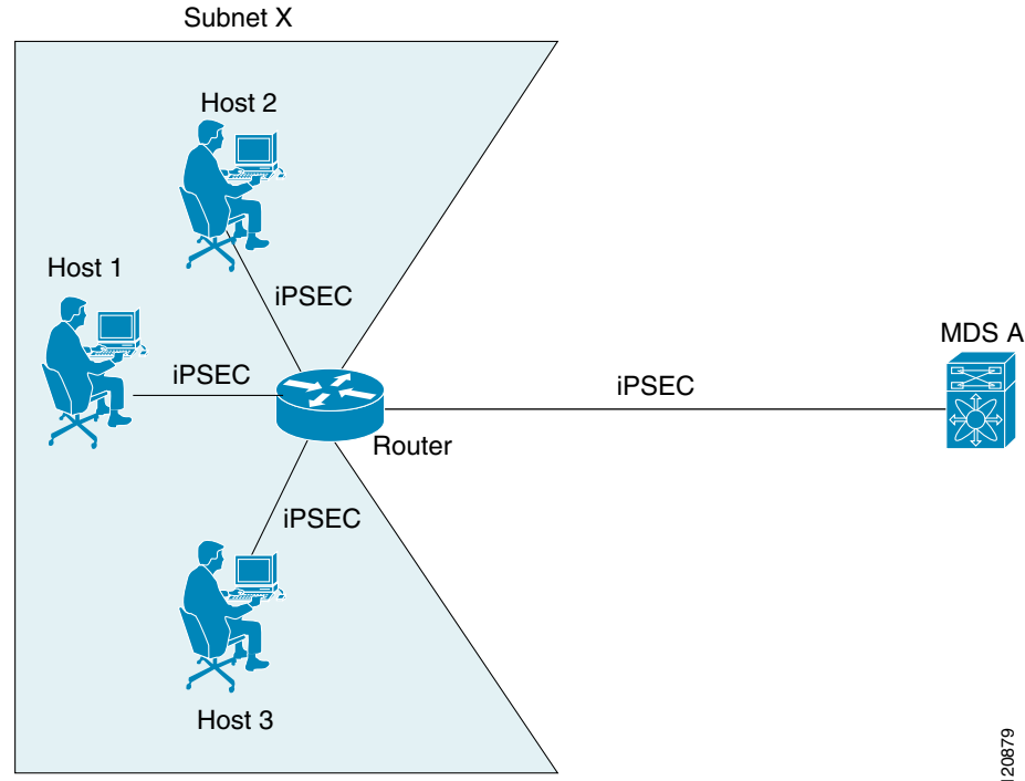
Figure 35-7 iSCSI with End-to-End IPsec Using the auto-peer Option
