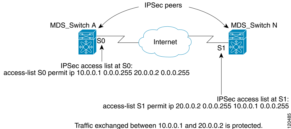
Figure 35-5 IPsec Processing of Crypto IPv4-ACLs
