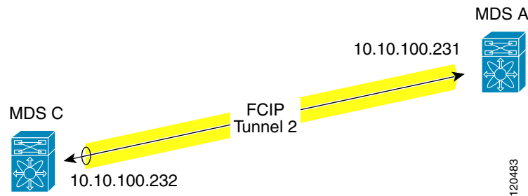
Figure 35-8 IP Security Usage in an FCIP Scenario
