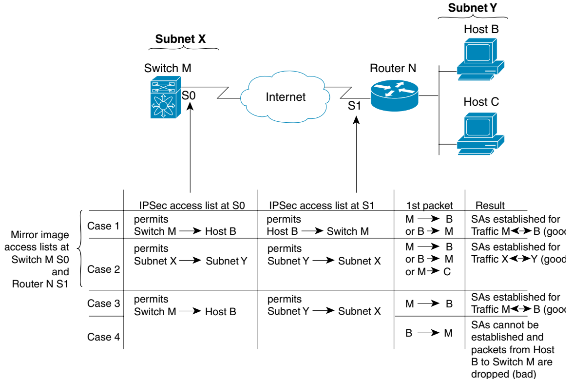
Figure 35-6 IPsec Processing of Mirror Image Configuration
