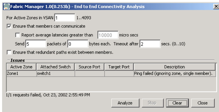
Figure 2-5 End to End Connectivity Analysis Window
