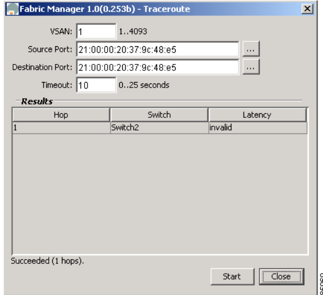
Figure 2-9 Traceroute Window
