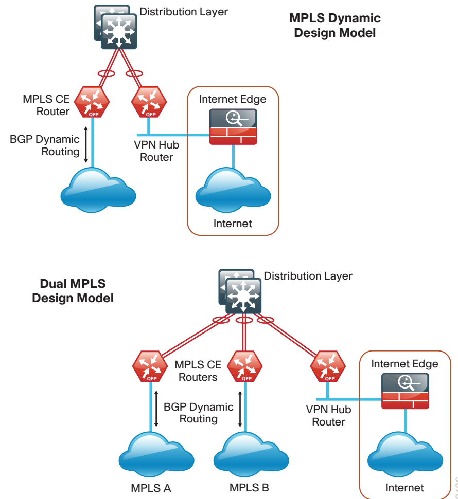
Figure 5 - DMVPN Backup Dedicated design model for MPLS WAN
