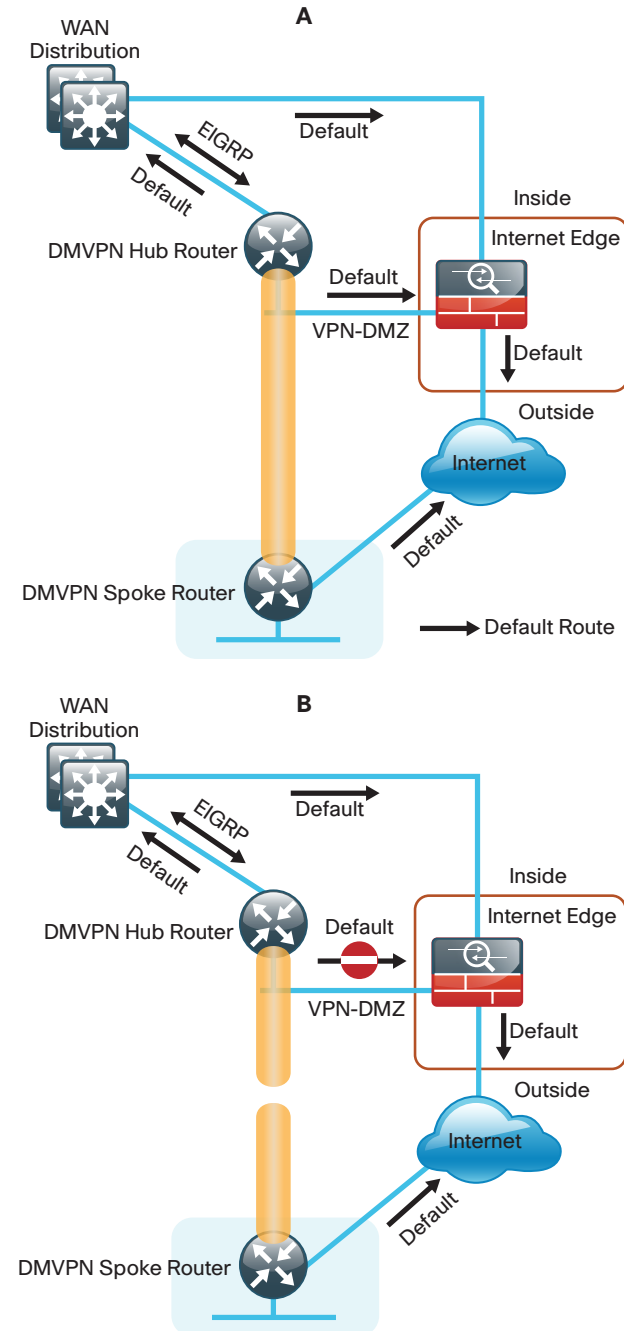
Figure 30 - IPsec tunnel before/after default route injection
