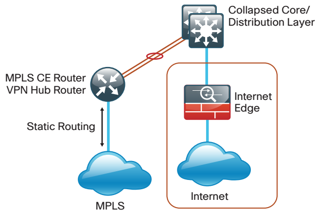
Figure 4 - DMVPN Backup Shared design model
