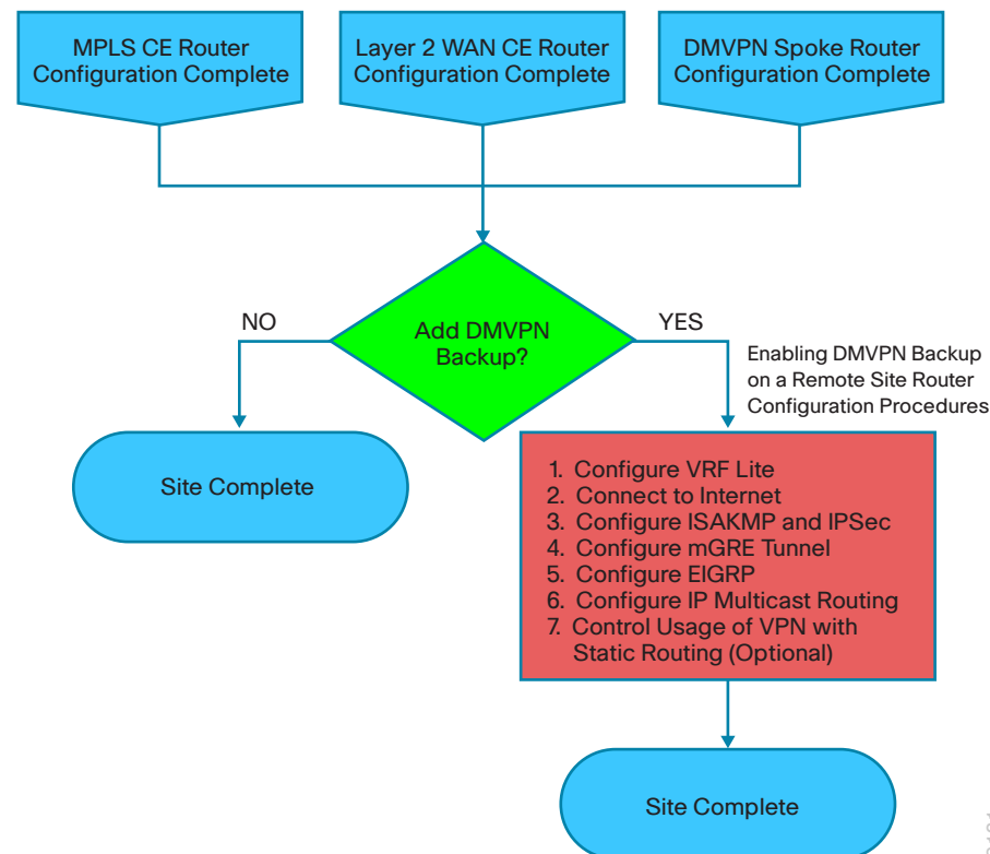
Figure 25 - Adding DMVPN Backup Configuration Flowchart
