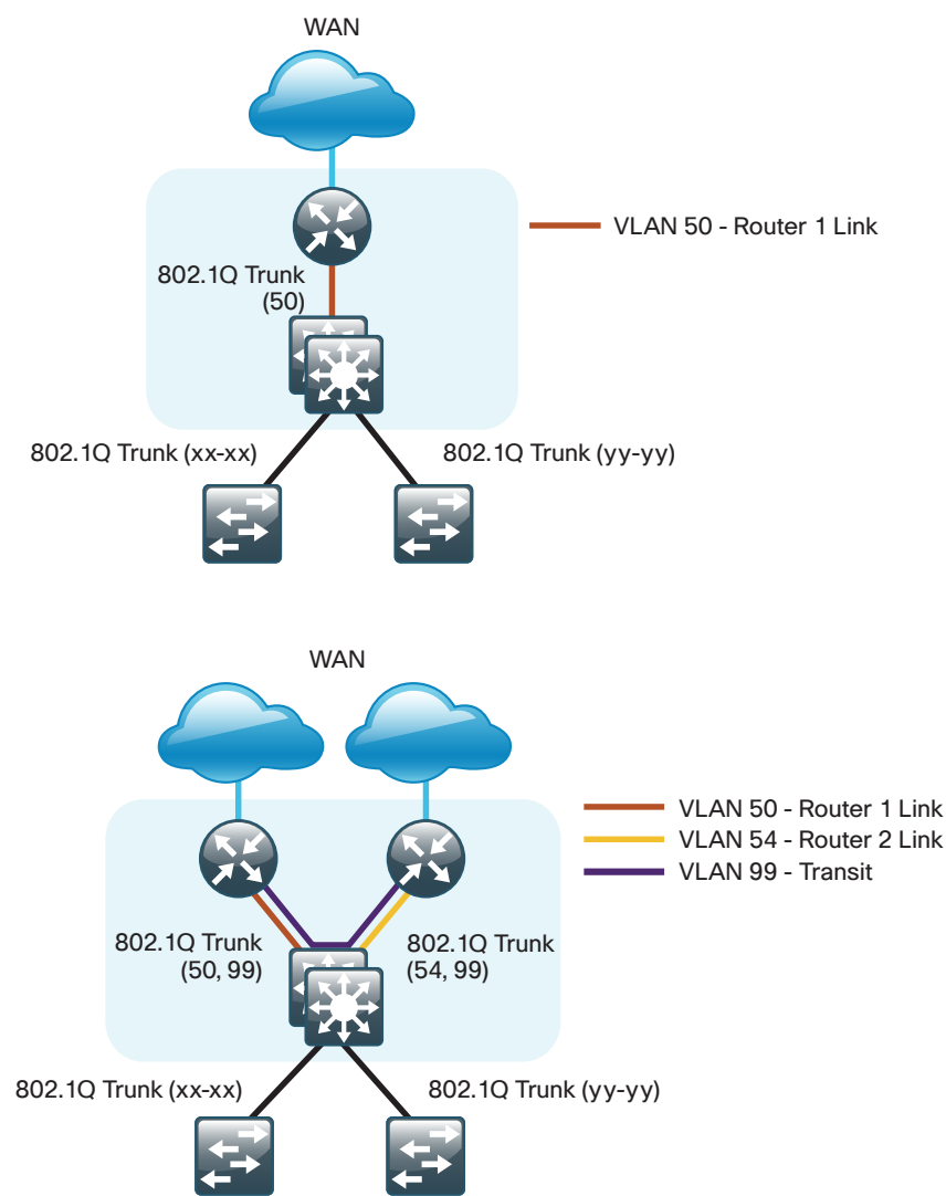
Figure 11 - WAN remote-site—Connection to distribution layer
