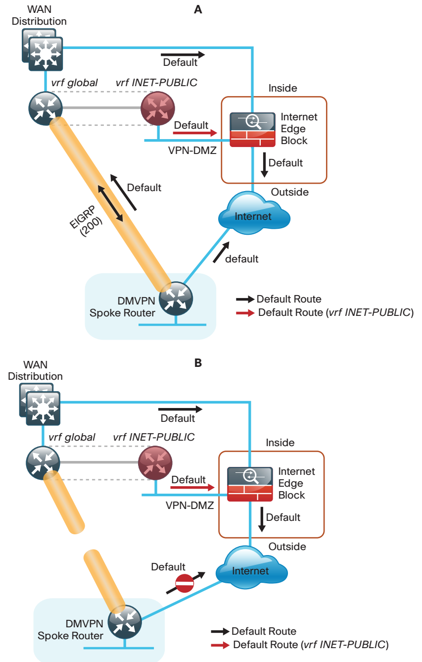
Figure 31 - IPsec tunnel with FVRF aggregation
