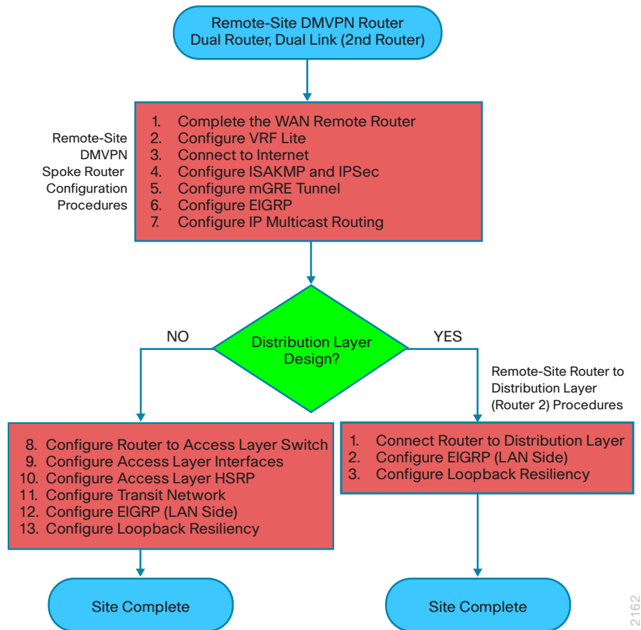
Figure 26 - Remote-site DMVPN spoke router configuration flowchart
