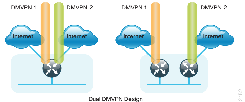
Figure 14 - DMVPN + DMVPN remote site (dual link options)
