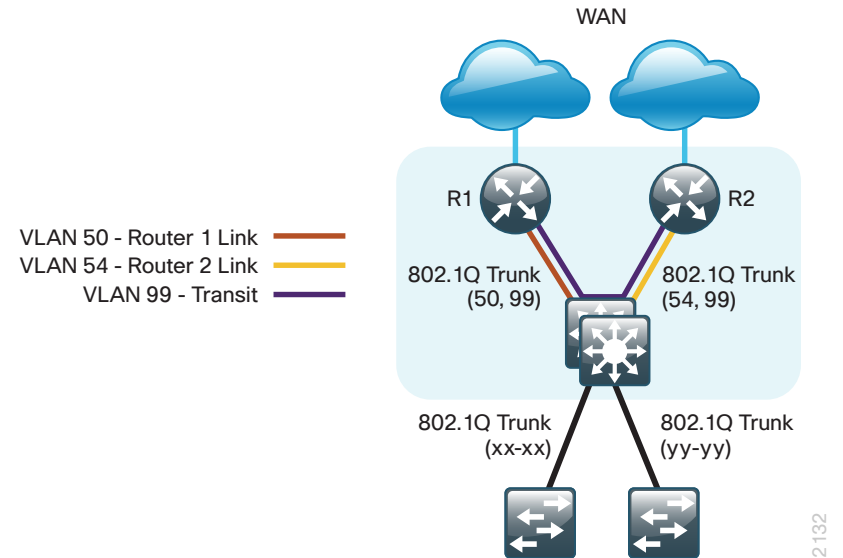
Figure 28 - WAN remote site - Connection to distribution layer
