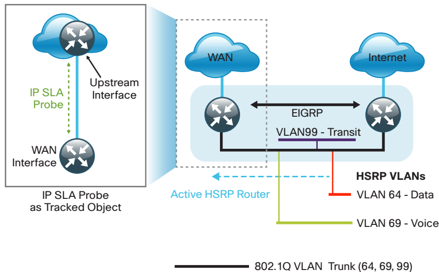
Figure 10 - WAN remote-site—IP SLA probe to verify upstream device reachability
