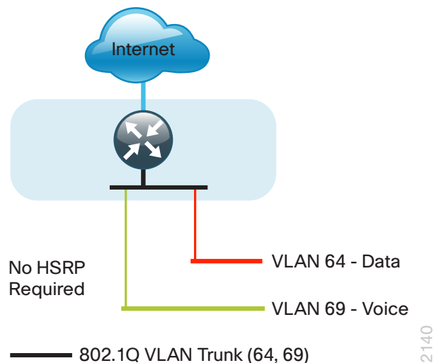
Figure 8 - WAN remote site—Flat Layer 2 LAN (single router)
