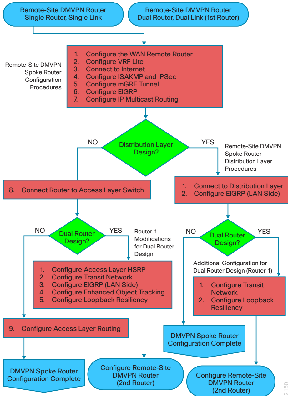
Figure 24 - Remote-site DMVPN spoke router configuration flowchart
