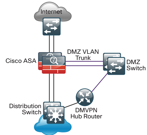
Figure 23 - DMZ VLAN topology and services
