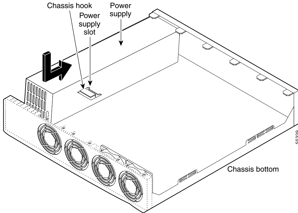
Figure 6-20 Inserting the Power Supply in the Chassis
