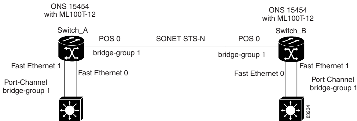
Figure 34-1 EtherChannel Example
