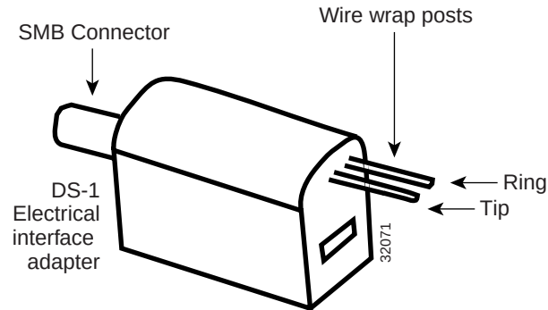
Figure 1-17 DS-1 Electrical Interface Adapter (Balun)
