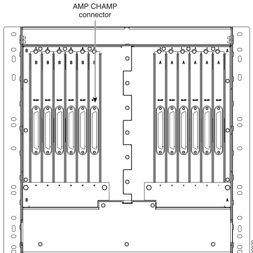
Figure 1-16 AMP EIA Champ Backplane
