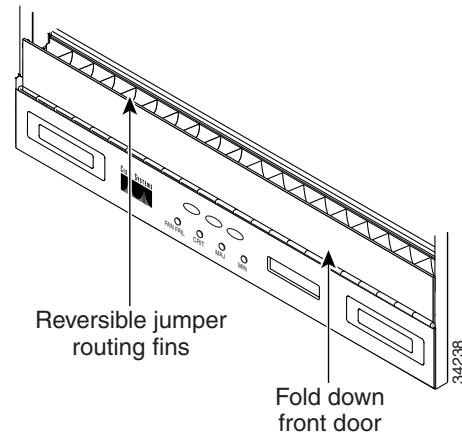
Figure 1-18 Managing Cables on the Front Panel
