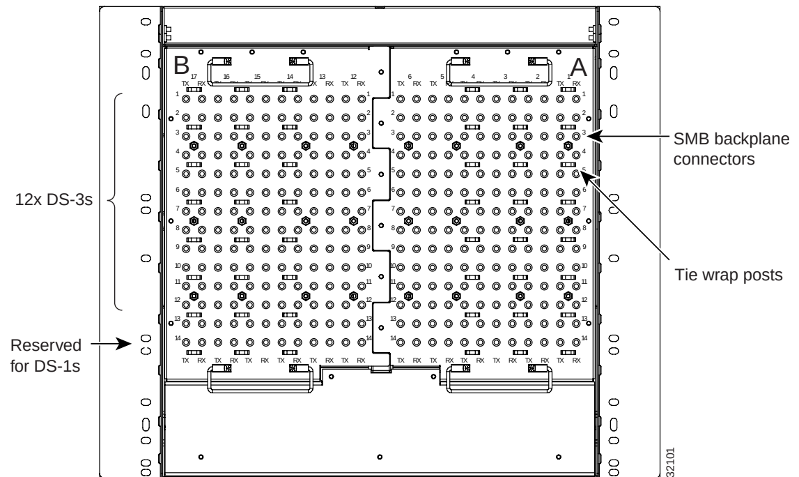
Figure 1-15 SMB EIA Backplane
