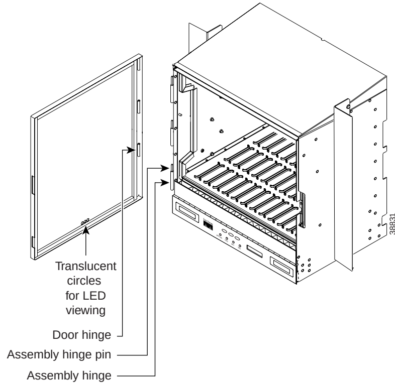
Figure 1-5 Removing the ONS 15454 Front Door
