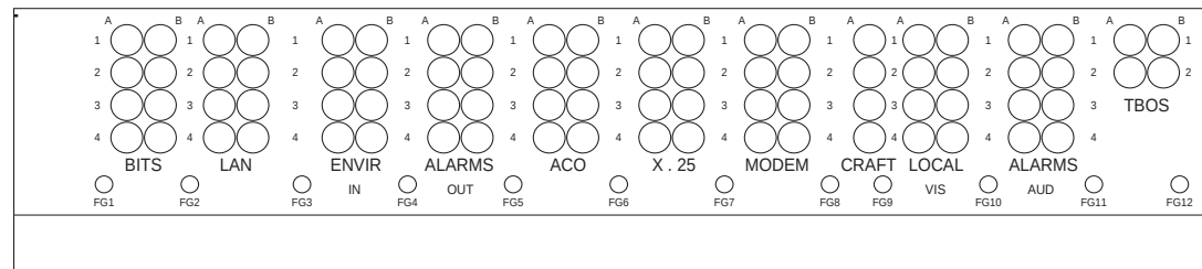
Figure 1-26 ONS 15454 Backplane Pinouts
