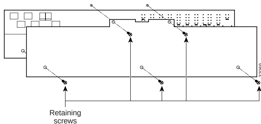
Figure 1-9 Removing the Lower Backplane Cover
