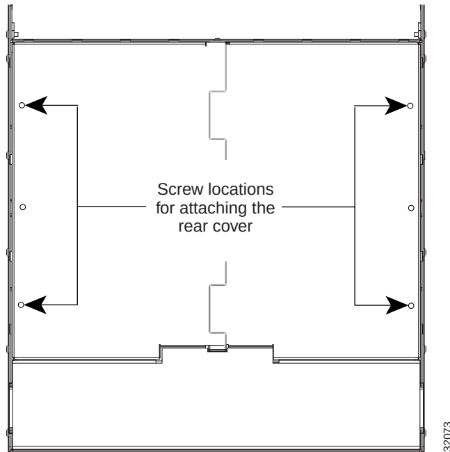
Figure 1-10 Backplane Attachment for Cover
