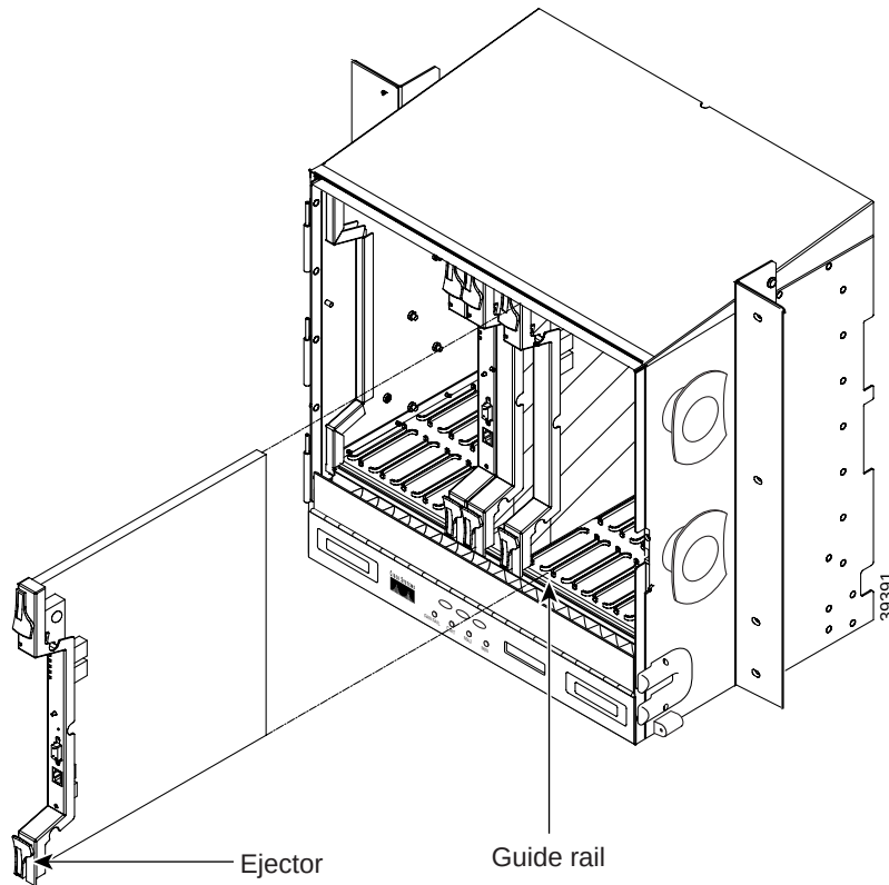
Figure 1-27 Installing Cards in the ONS 15454
