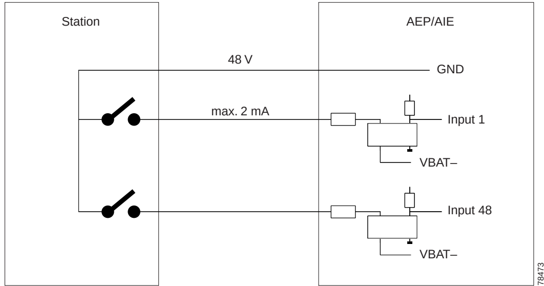
Figure 1-22 Alarm Input Circuit Diagram
