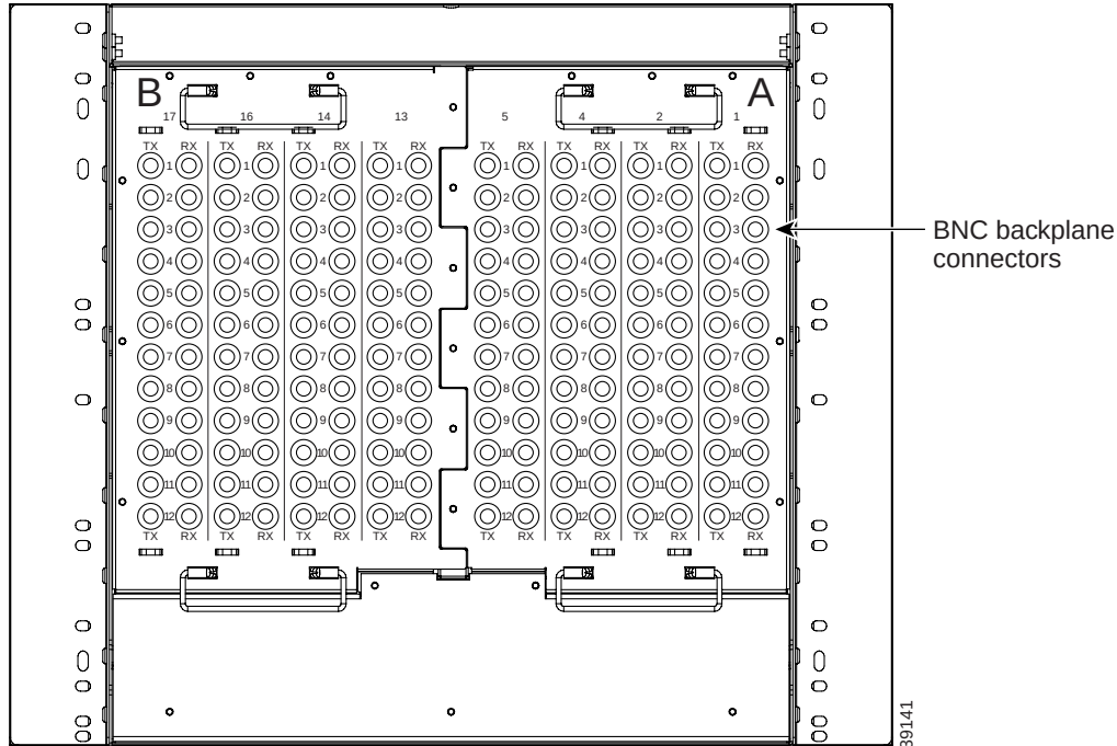
Figure 1-14 High-Density BNC Backplane for use in 1:N Protection Schemes
