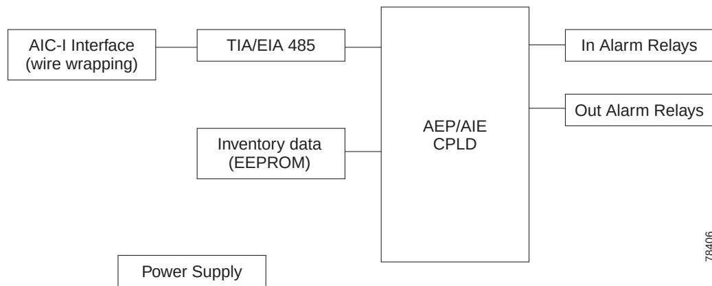
Figure 1-20 AEP Block Diagram
