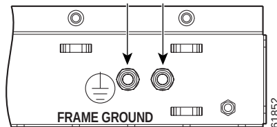
Figure 1-24 Ground Posts on the ONS 15454 Backplane
