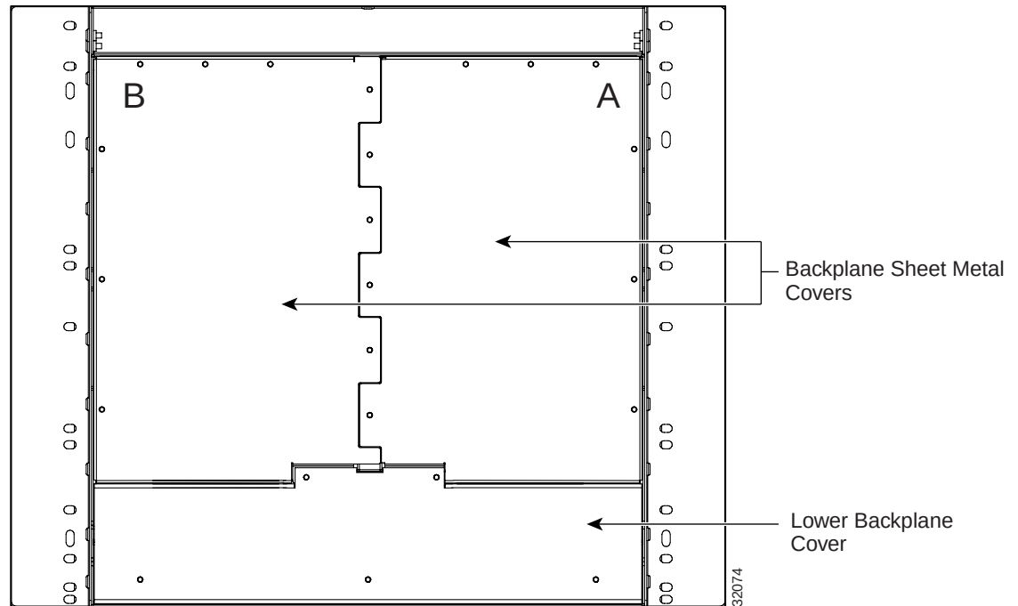
Figure 1-8 Backplane Covers
