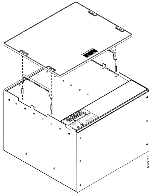
Figure 1-11 Installing the Plastic Rear Cover with Spacers
