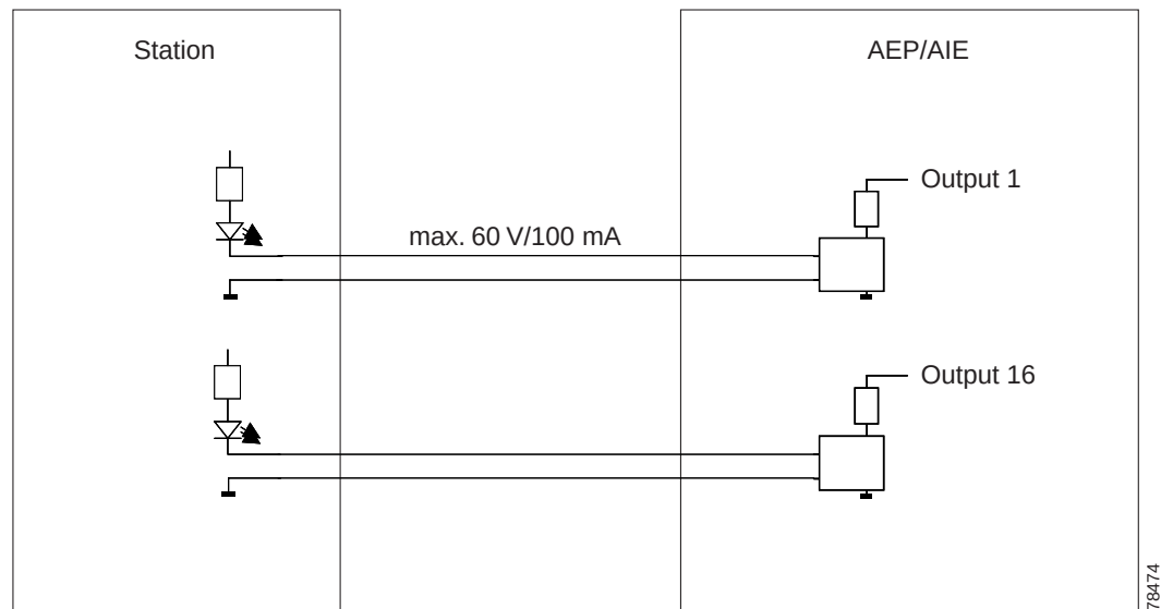
Figure 1-23 Alarm Output Circuit Diagram
