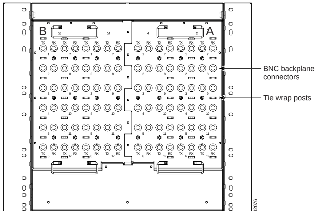
Figure 1-12 BNC Backplane for use in 1:1 Protection Schemes
