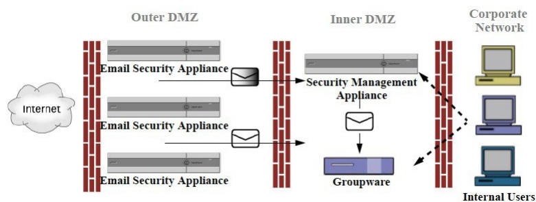
Figure 86: Typical Network Configuration with Cisco Content Security Management Appliance
