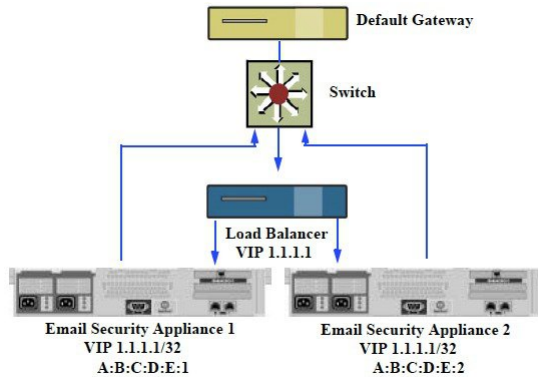
Figure 75: Using DSR to Load Balance Between Multiple Appliances on a Switch
