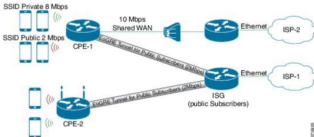
Figure 17: EoGRE Downstream QoS Use Case
