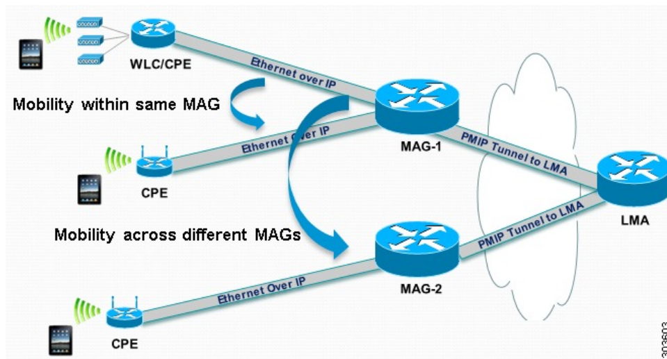
Figure 5: Structure of the EoGRE Deployment with PMIPv6 Integrated for Mobility Service
