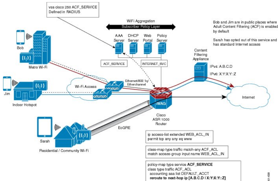
Figure 14: Adult Content Filtering on Wi-Fi Hotspots
