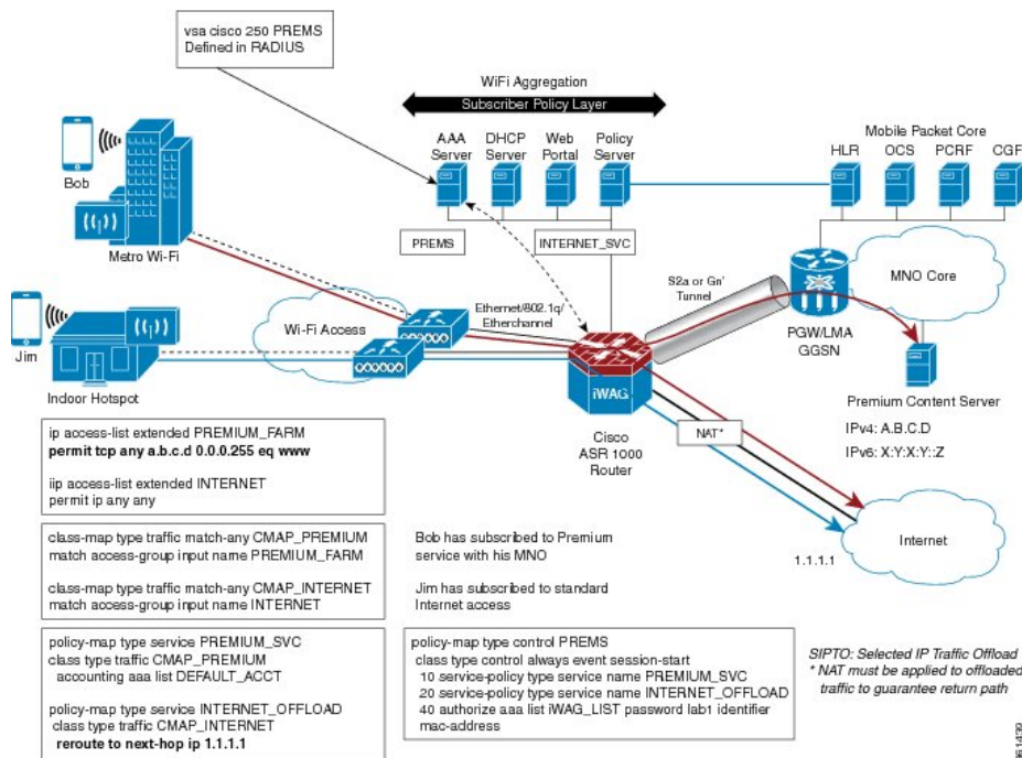
Figure 15: Flow-Based Redirect for Selective IP Traffic Offload
