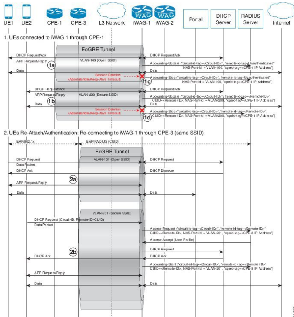
Figure 21: EoGRE Intra-iWAG Roaming and Restart With Same SSID Call Flow
