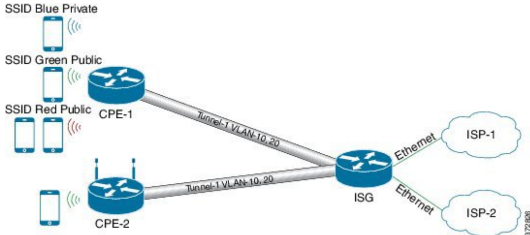
Figure 19: Single Tunnel for Multiple SSIDs
