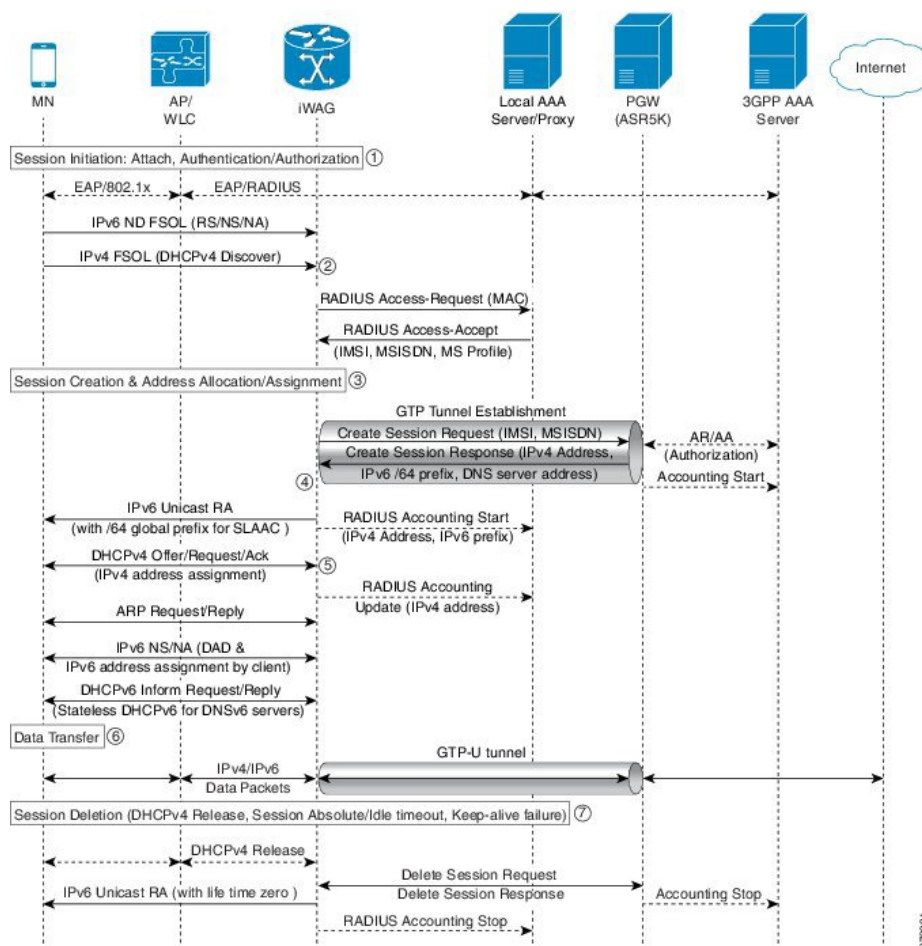
Figure 13: Dual-Stack Mobile IPoE Session for GTPv2 Call Flow
