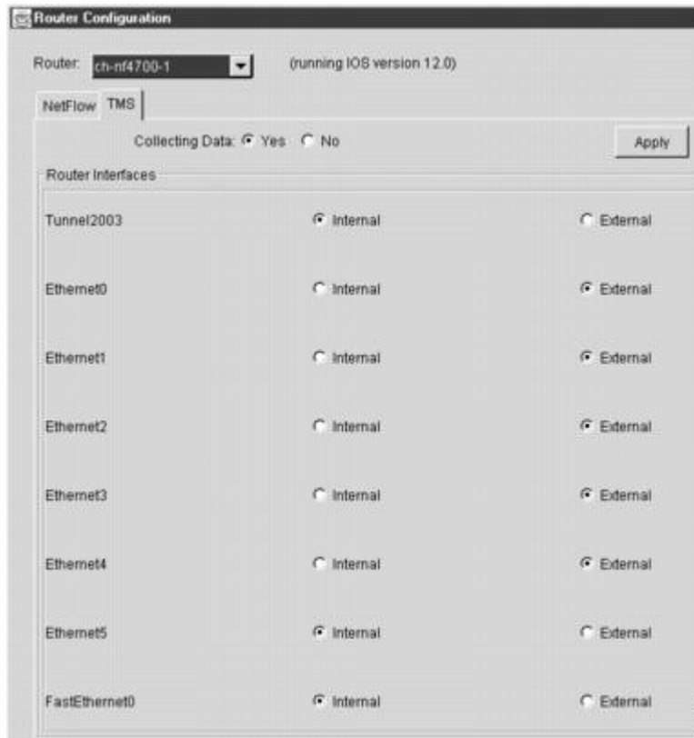
Figure 6: Setting the NDA Configuration Window
