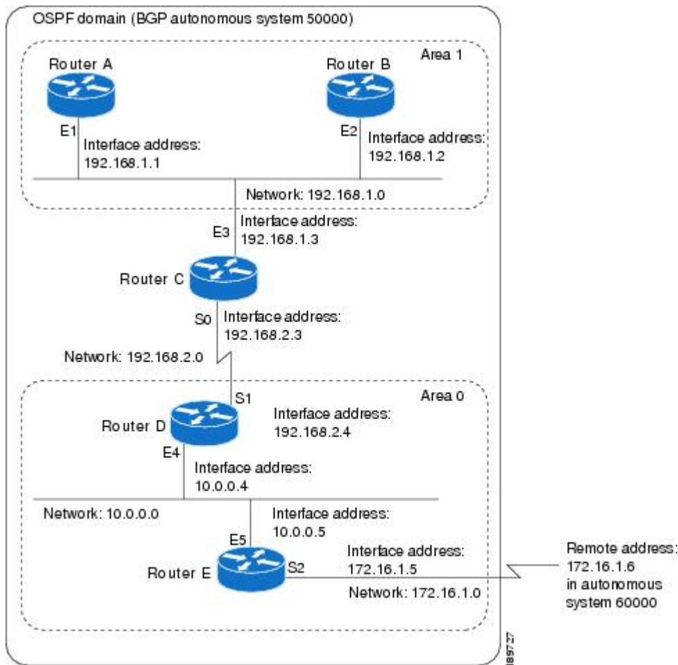
Figure 5: Sample OSPF Autonomous System Network Map
