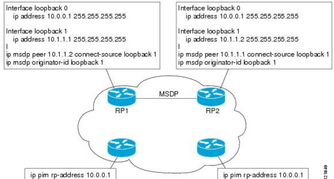
Figure 8: AnyCast RP Configuration
