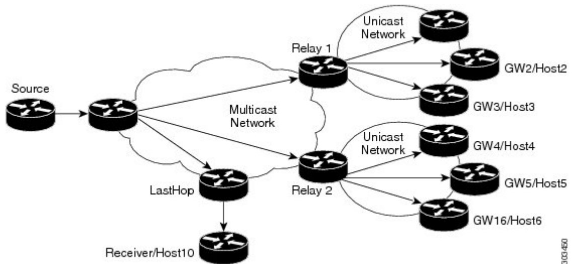
Figure 16: Automatic Multicast Tunneling (AMT)
