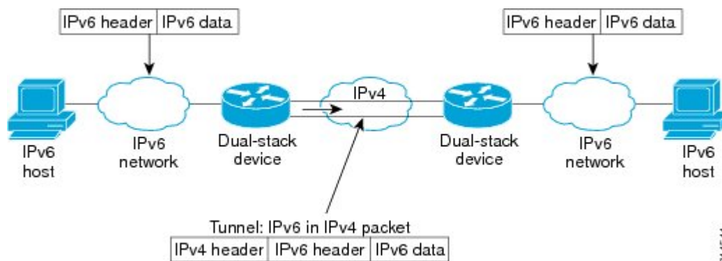
Figure 7: Overlay Tunnels
