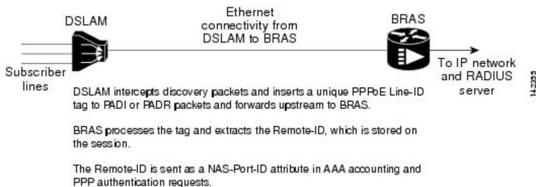
Figure 9: PPPoE Circuit-Id Tag Processing Solution
