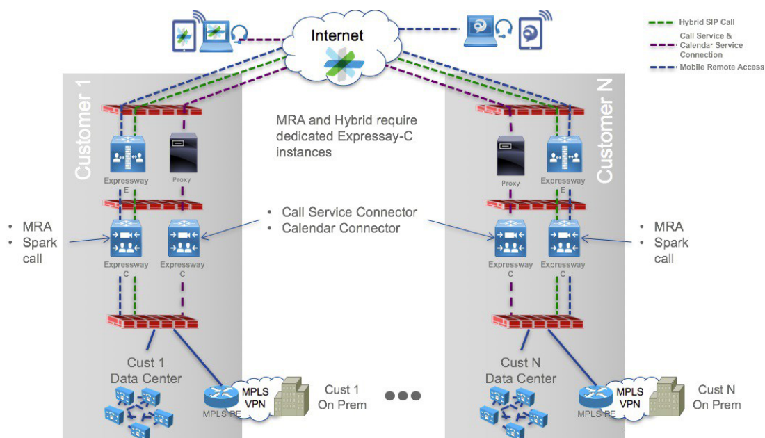
Figure 15 Single-tenant VCS deployment
