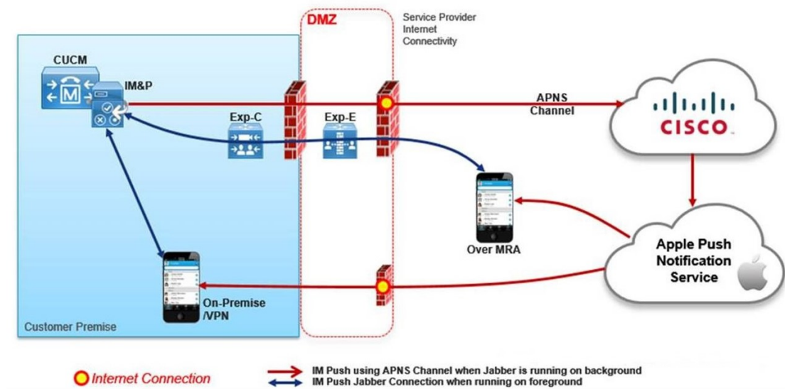
Figure 17 Apple Push Notifications for Unified CM IM&P and Jabber iOS
