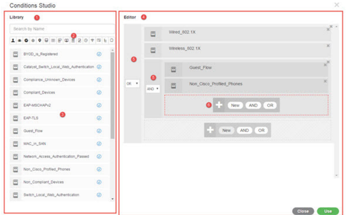
图 42: Conditions Studio
