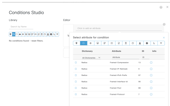
图 61: Conditions Studio
