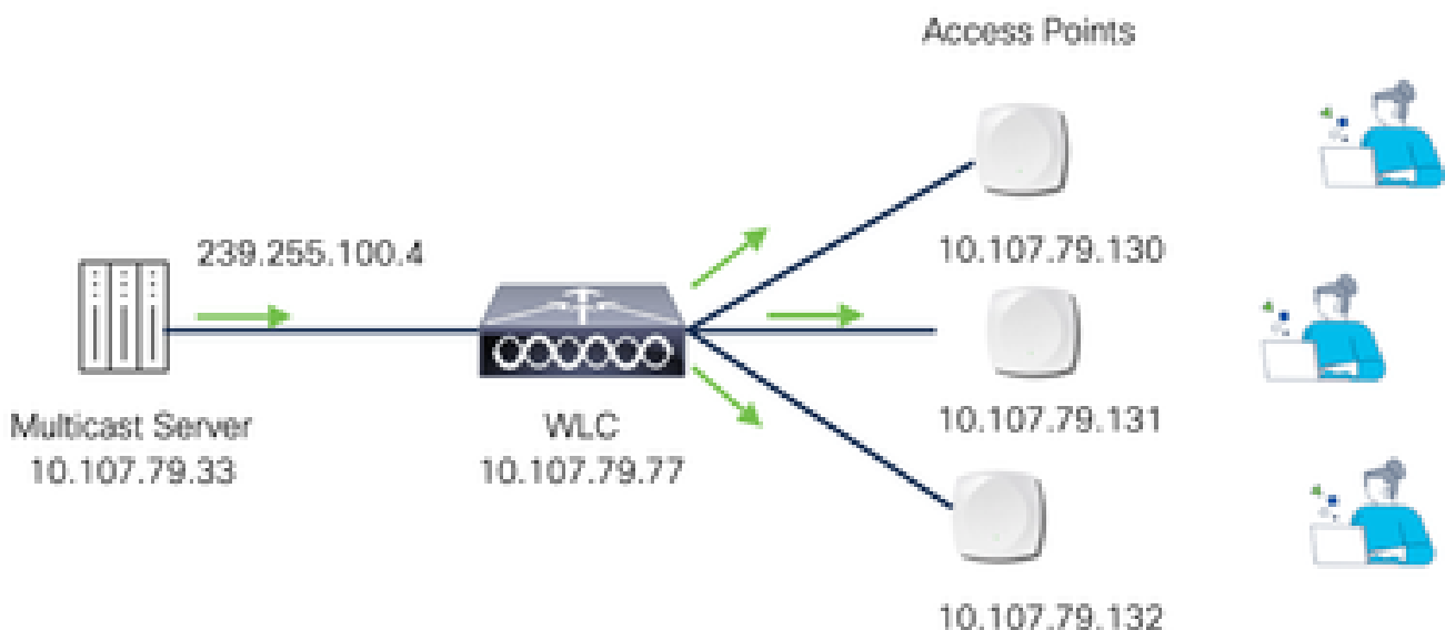
Multicast-over-Unicast
