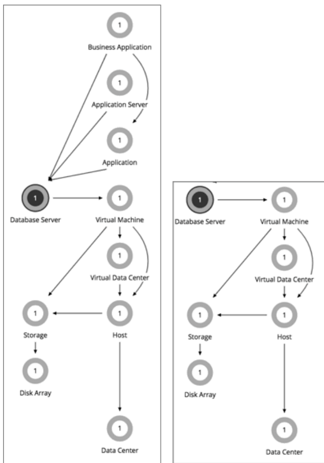
AppDynamics
