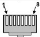
RJ-45 Alarm Connector on IE-4010 Chassis
