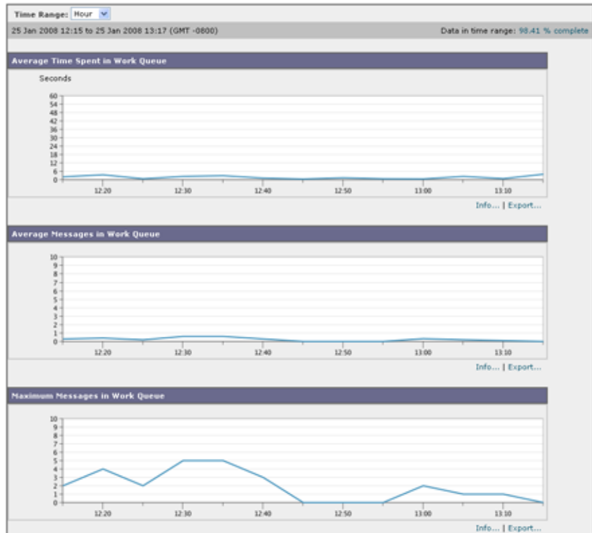
図 2-30 [System Capacity] : [Workqueue]
