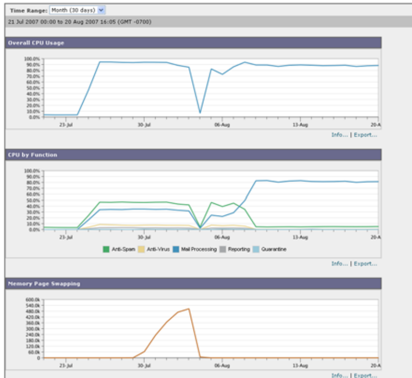
図 2-35 [System Capacity] : [System Load]
