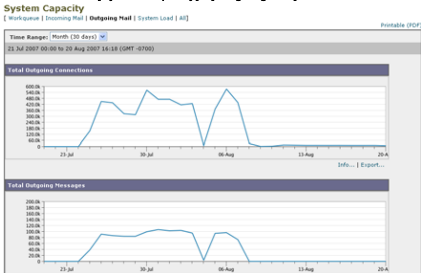
図 2-33 [System Capacity] : [Outgoing Mail] (1/2 ページ)
