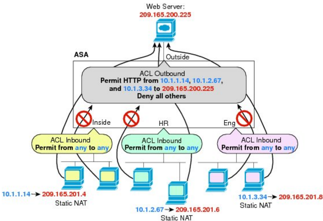
図 1: Outbound ACL
