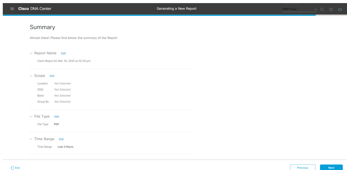
図 32: [Summary]
