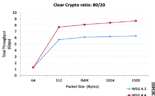
Line chart for max throughput comparison between release 4.3 and 4.4 for 80/20 traffic
