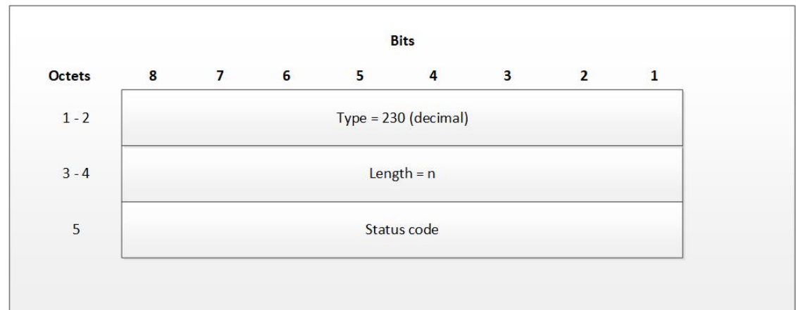
Figure 19: Subscriber Trace Status Report
