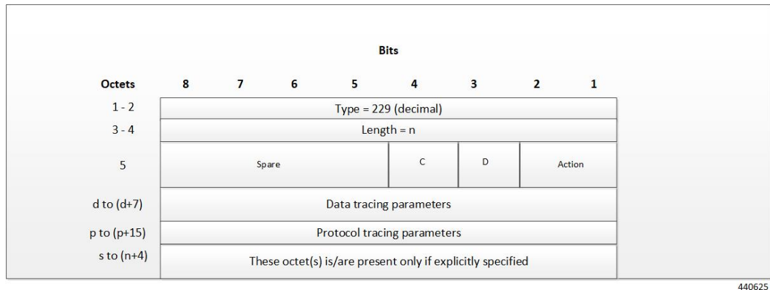
Figure 17: Subscriber Tracing
